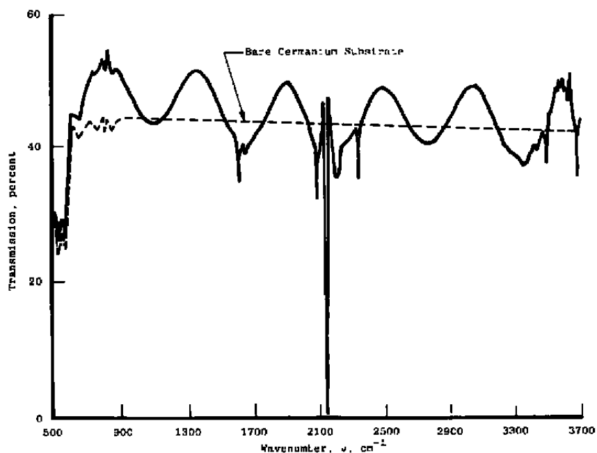
Figure 19. Transmittance of 6.54- \mu\text{m} -thick solid \text{CO}/\text{H}_2\text{O} mixture (91%/9%) on 20°C germanium.
