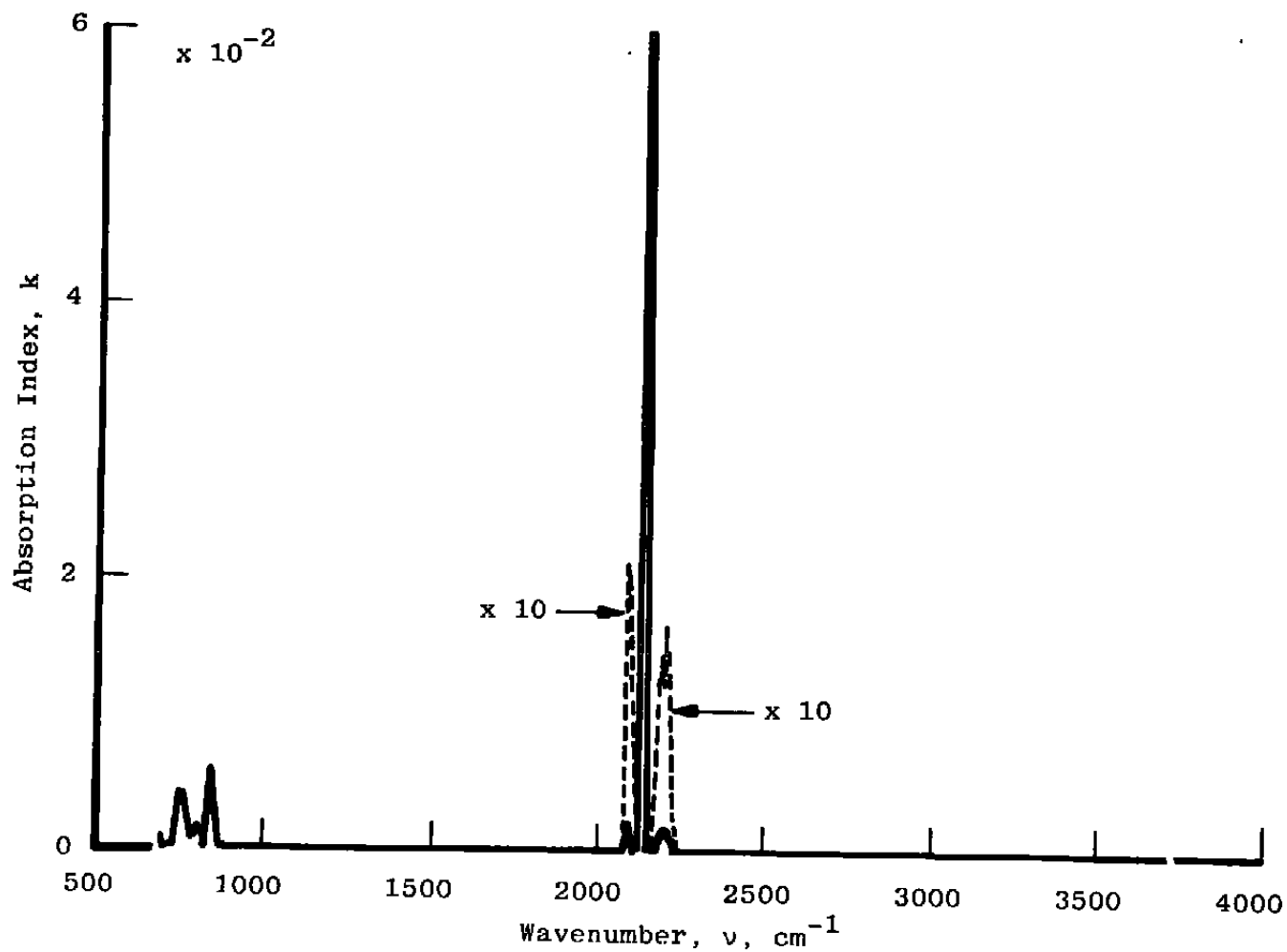
Figure 28. Absorption index of solid \text{N}_2/\text{CO} mixture (79%/20%) on 20^\circ\text{K} germanium.
