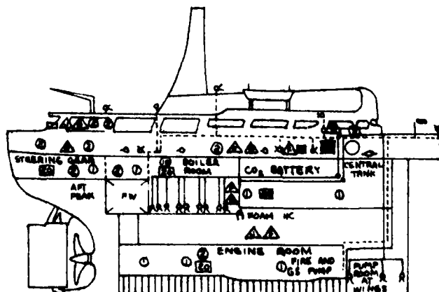
FIRE FIGHTING PLAN FOR THE AFT END OF A SUPER TANKER.
