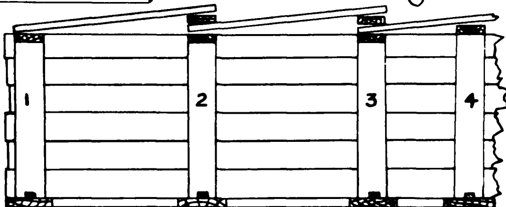
TYPICAL SECTION
