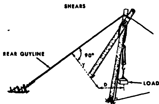
Ginpole and shears.
