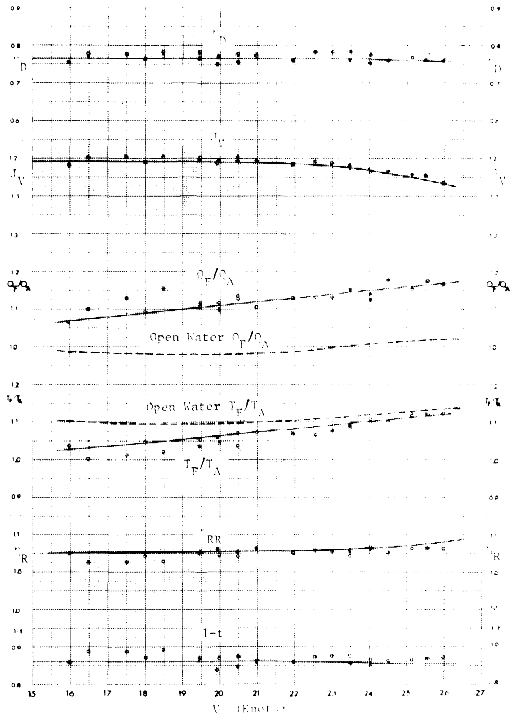
Figure 38 - Data and Fitted Curves from the Series of T_F/T_A Experiments with Model 5362 at the Full Scale, Re = 1.5 \times 10^6 , compared with the LIPS Design Contract Data, Re = 1.5 \times 10^6 , Pr = 0.71 .
