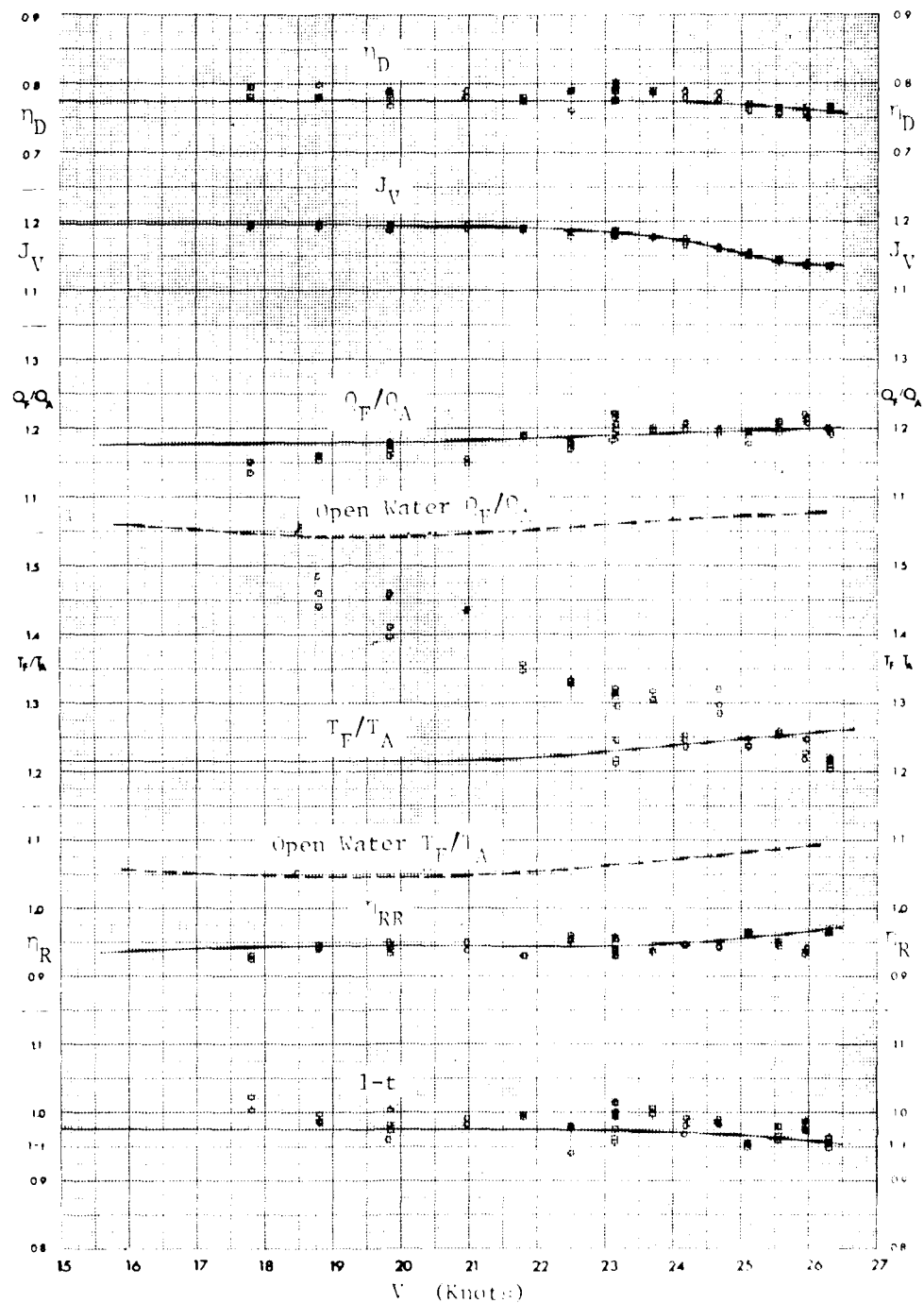
Figure 42 - Data and Faired Curves from the April 1966 Experiments with Model 5362 at the Full Load displacement. Fitted with the JIPS Design Contraints in the JIPS Design Program 020 in the DPM500 Propeller Design Program.
