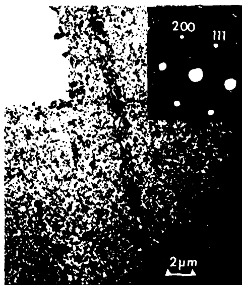
Figure 6. Abnormal grain in as hot-worked MA 753. Long direction of the grain is parallel to \langle 200 \rangle is parallel to the working direction. Zone axis is \langle 01\bar{1} \rangle . 120 kv.
