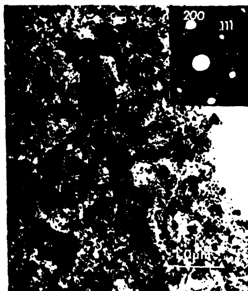
Figure 7. Different abnormal grain from the same specimen as Figure 6 . Long direction of the grain is parallel to \langle 200 \rangle is parallel to the working direction. Zone axis is \langle 01\bar{1} \rangle . 120 kv.
