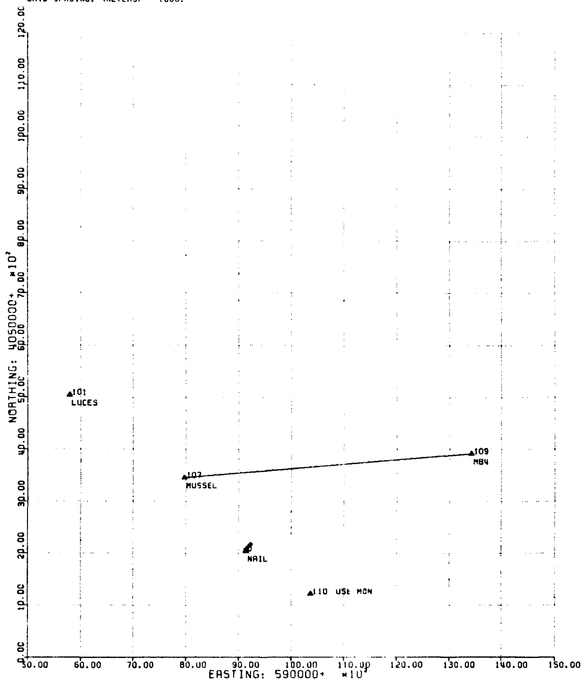
Figure 9. Pier Test (MRS III Data)
