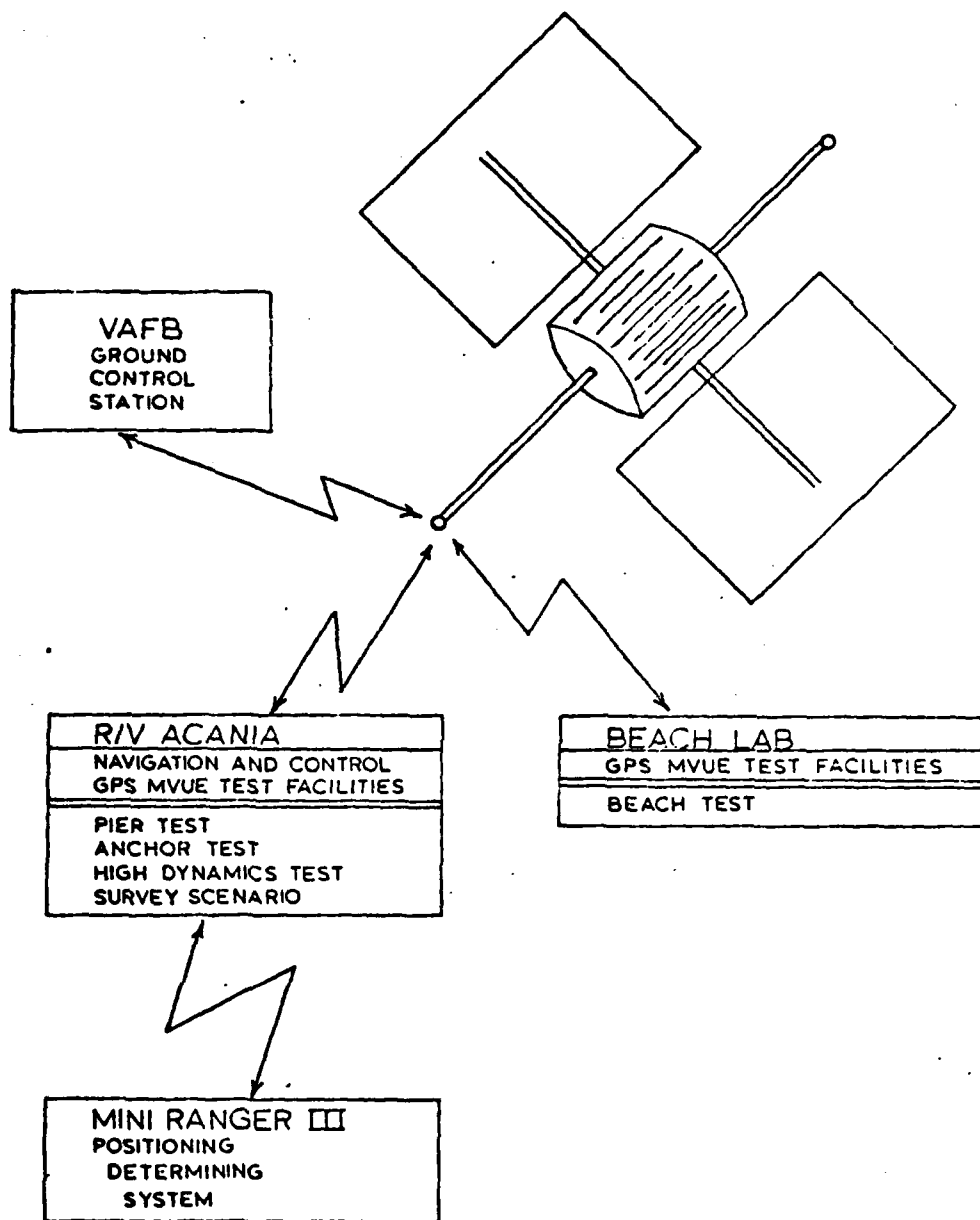
FIGURE 3-2. ACANIA/MVUE GPS SYSTEM TEST CONFIGURATION
