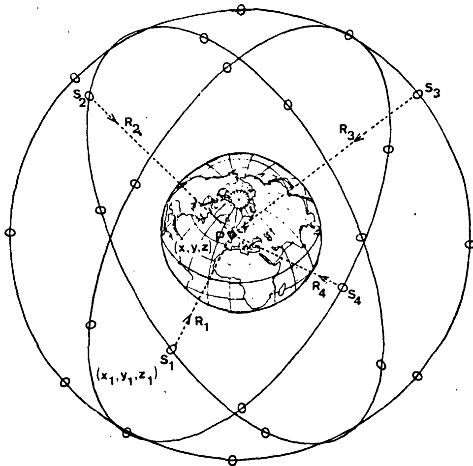
Figure 1. GPS Earth Centered Coordinate System
