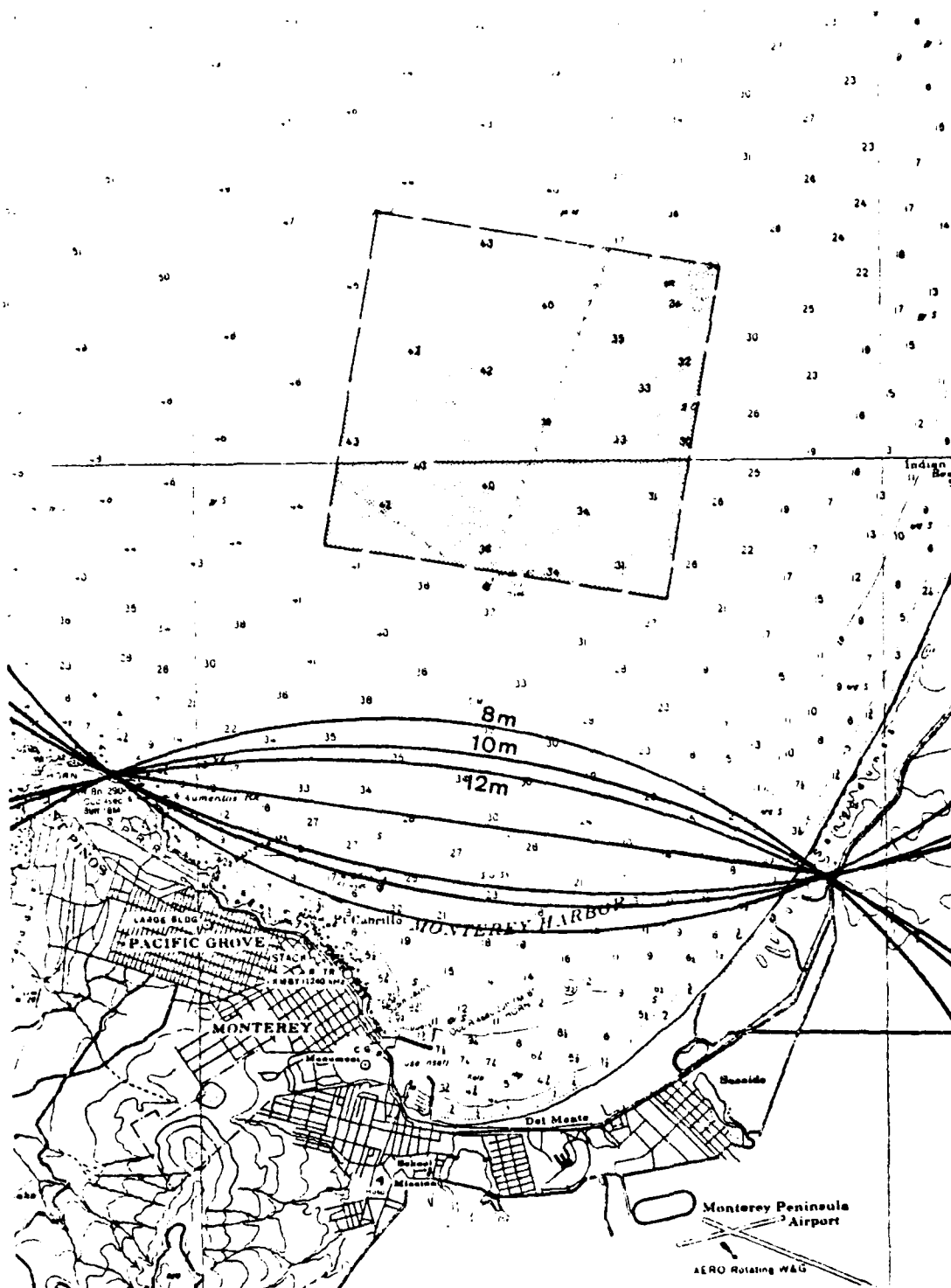
Figure 23. Two d_{rms} Repeatability Contours (Luces Pt. and Monterey Bay 4 Operating Area)
