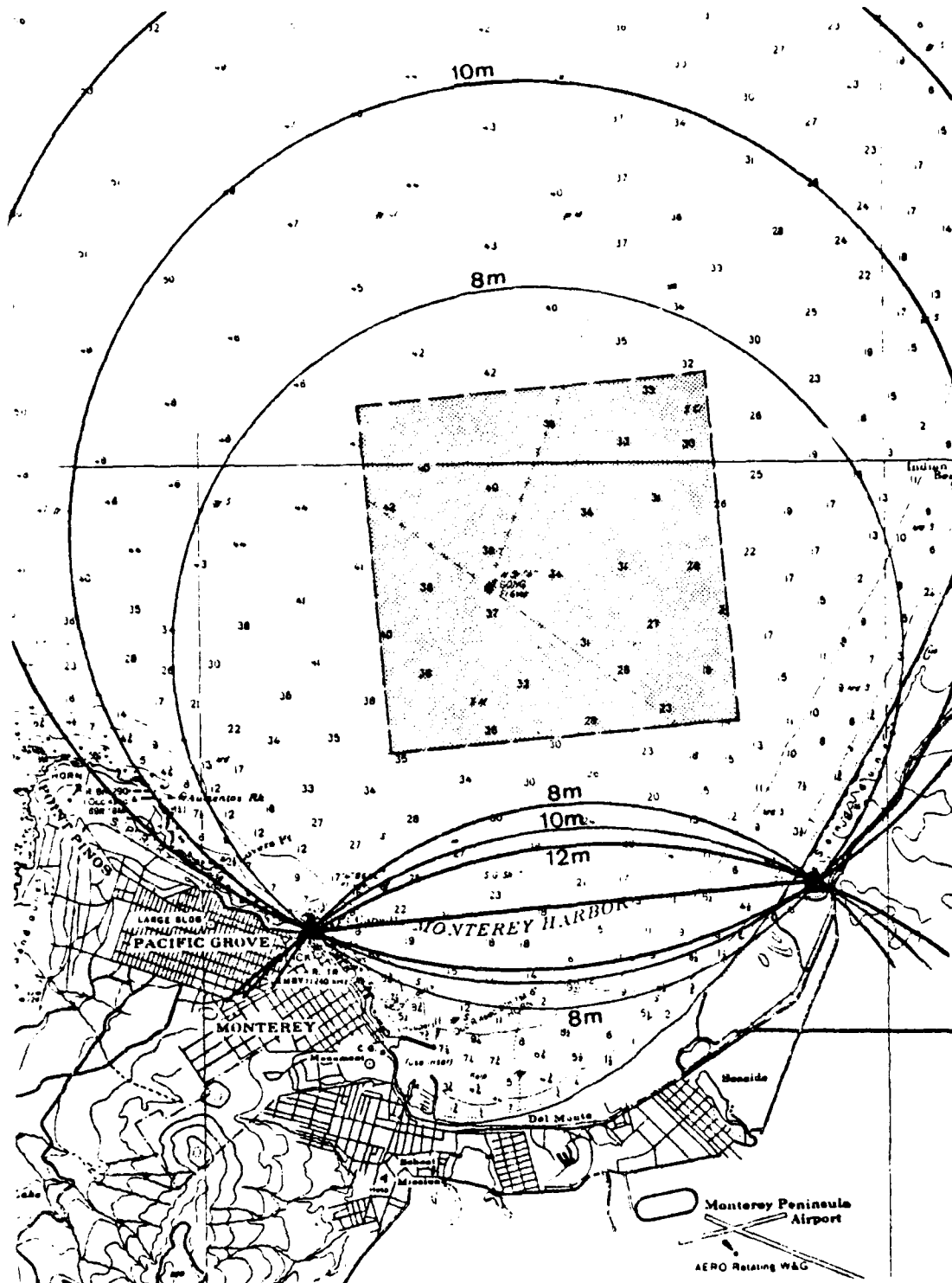
Figure 22. 2 d_{rms} Repeatability Contours (Mussel and Monterey Bay 4 Operating Area)
