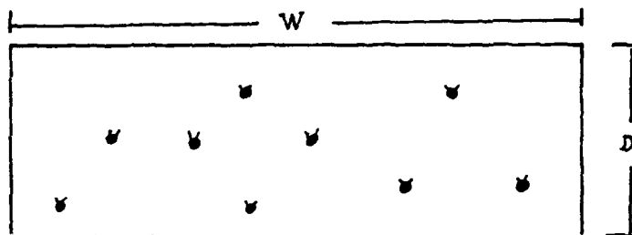
Figure 1. Mine Field Model
