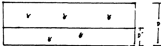
Figure 4. Location of D'
