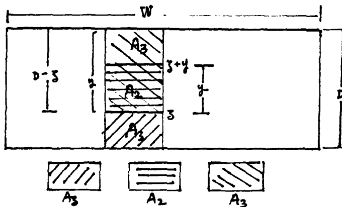
Figure 2. Area of a Path
