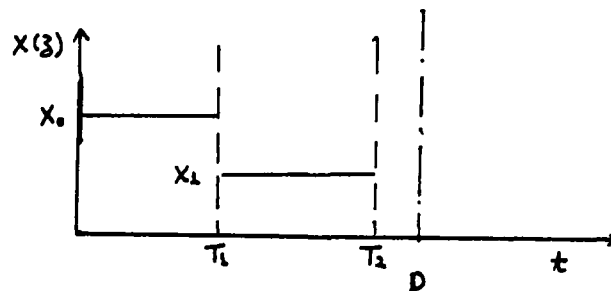
Figure 3. Distribution of T_i 's
