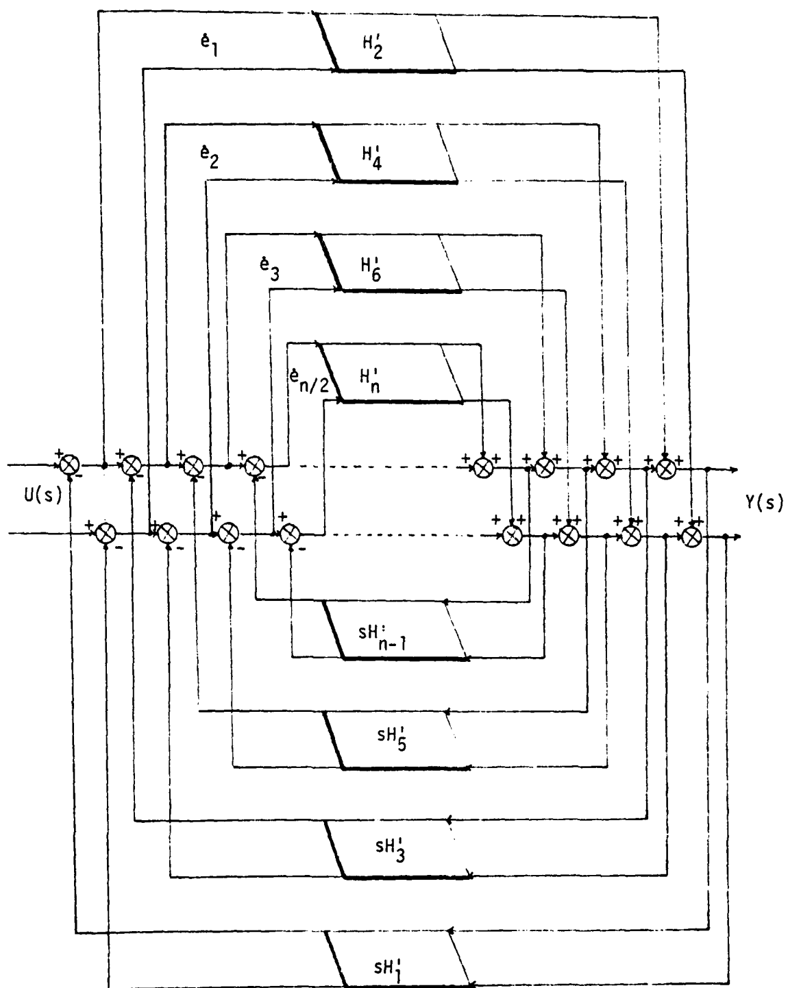
Figure 3. Matrix representation of a n th/2 order system by Cauer first form with two inputs two outputs. ( n even)
