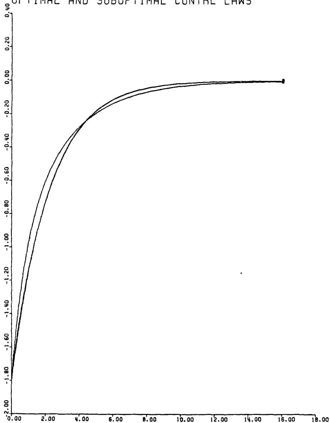
FIG. 18 - EXAMPLE 3.1 - NEAR OPT. SOLUTION OPTIMAL AND SUBOPTIMAL CONTRL LAWS
