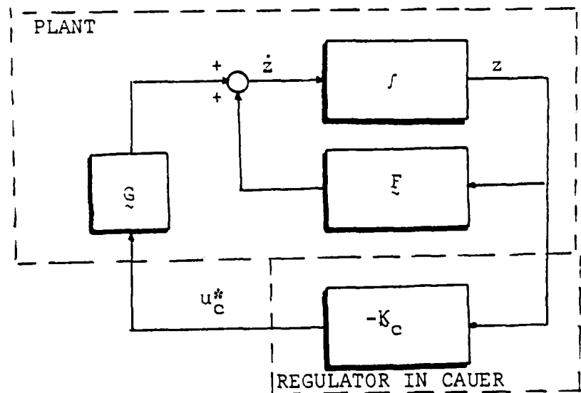
Figure 15. Linear Regulator in Cauer Form.
