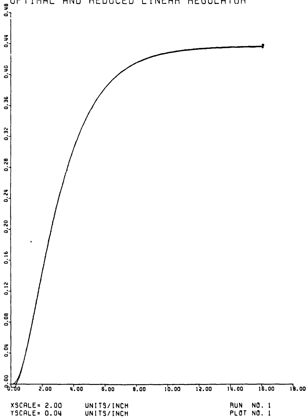
FIG. 17 - EXAMPLE 3.1 STEP RESPONSE OPTIMAL AND REDUCED LINEAR REGULATOR
