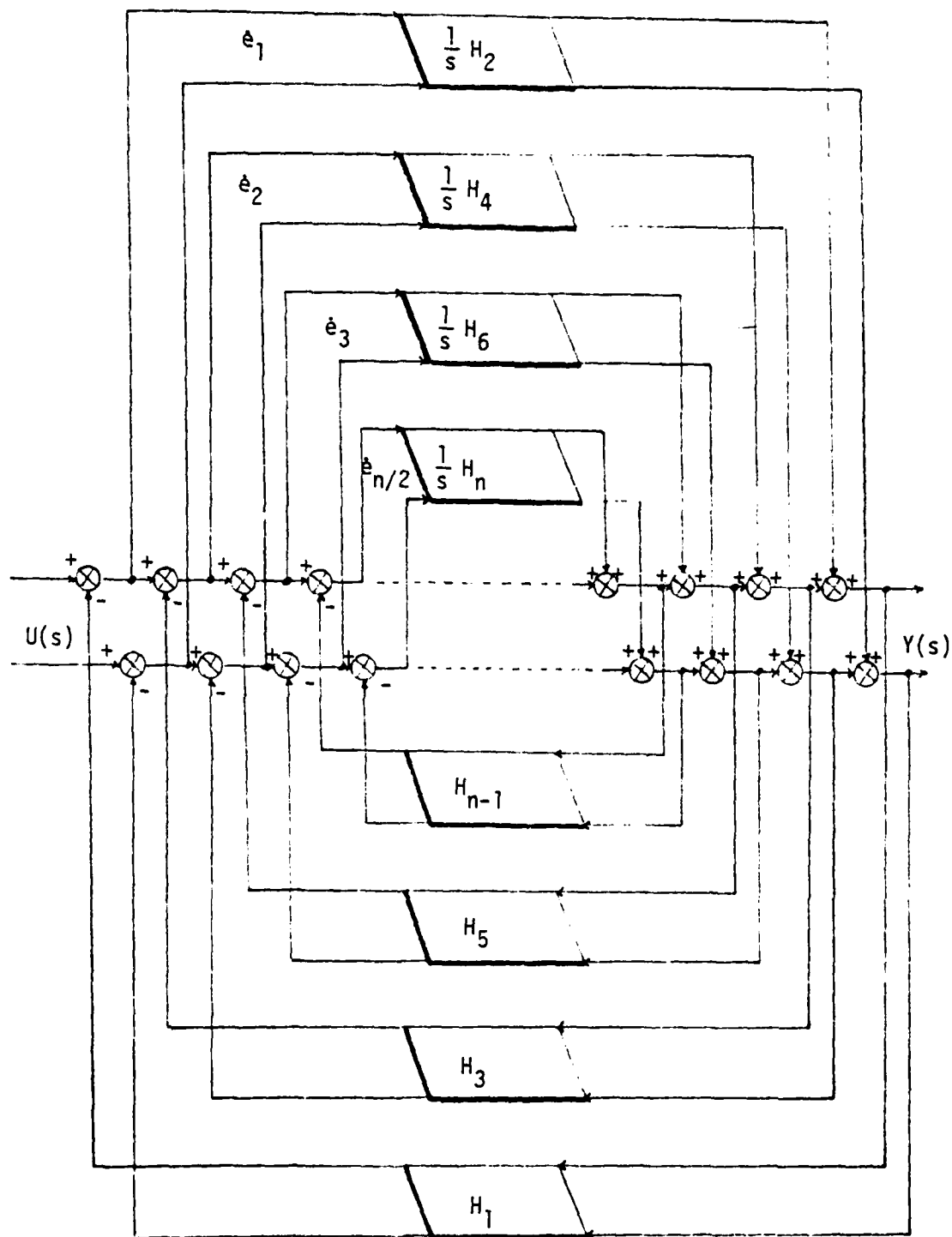
Figure 4. Matrix representation of a n/2 order system by Cauer second form with two inputs two outputs. ( n even)
