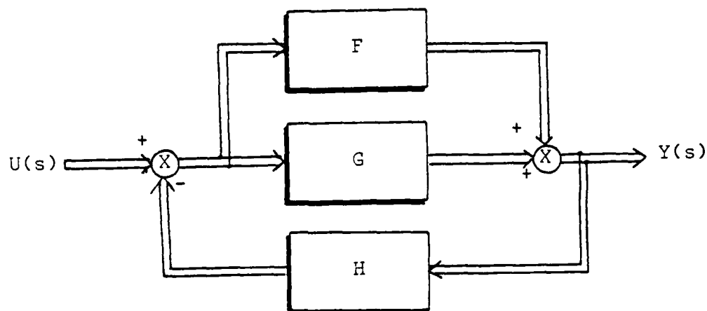
Figure 1. Feedback and Feedforward controls.
