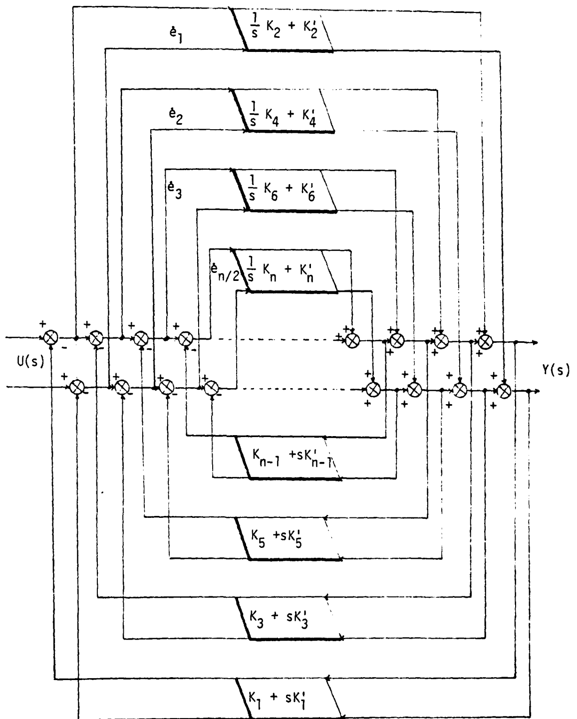
Figure 2. General Matrix representation of a n th order system by Causer mixed form with two inputs two outputs. ( n even)
