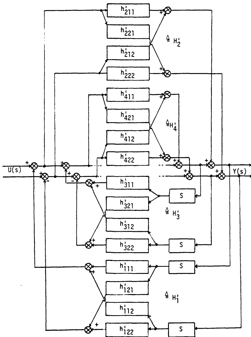
Figure 8. Simulation diagram for fourth order system with m = 2 for Caier matrix first form.
