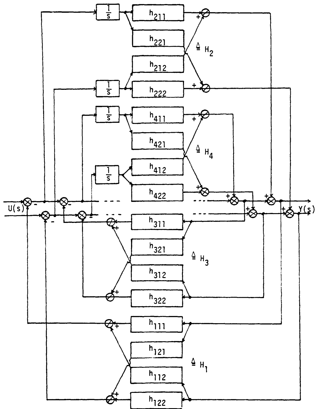
Figure 9. Simulation diagram for fourth order system with m = 2 for Cauer matrix second form.
