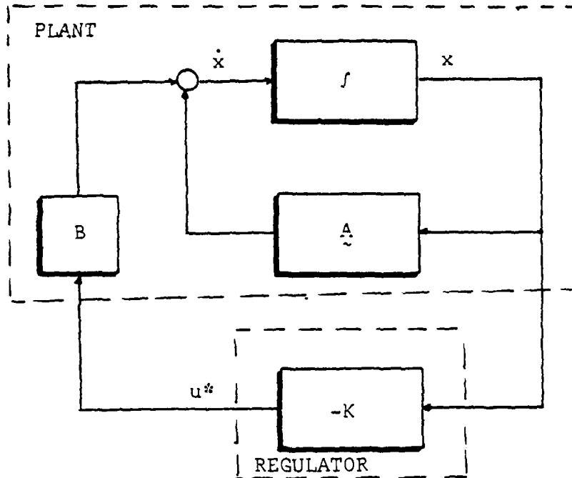
Figure 14. Linear Regulator System
