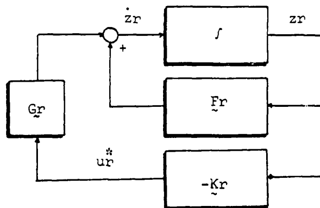
Figure 16. Reduced Linear Regulator in Cauer Form
