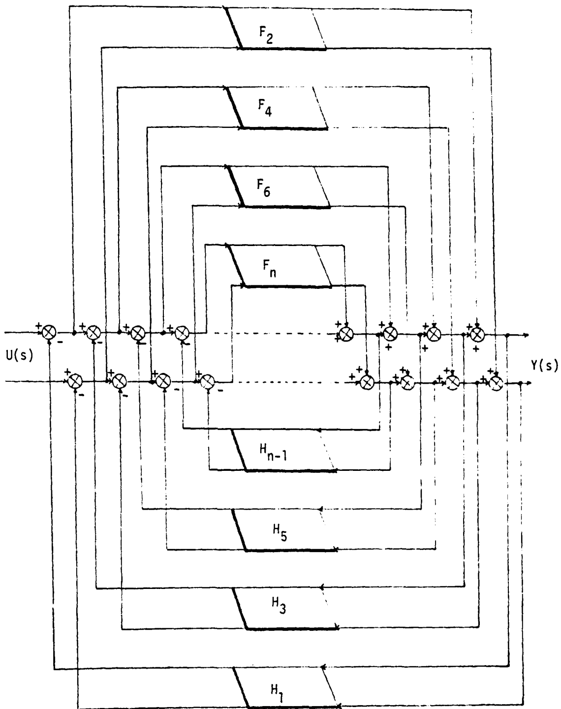
Figure 6. Block diagram representation of a continued fraction expansion.
