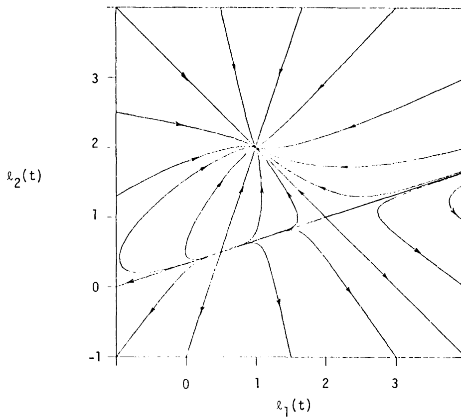
Figure 5: The phase plane for the Riccati solution components for Example 1.
