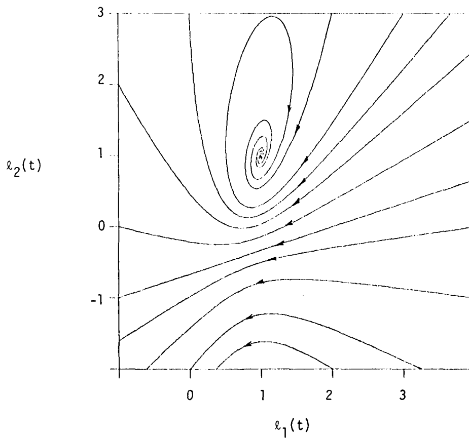
Figure 6: The phase plane for the Riccati solution components for Example 2.
