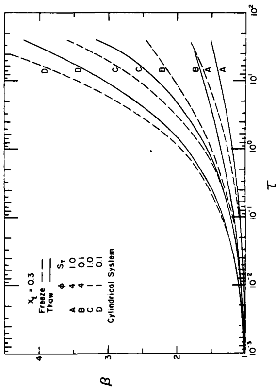
Figure 8. Phase change position vs time x_0 = 0.3 .
