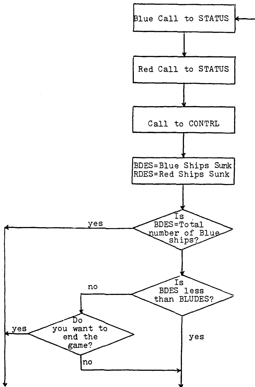
Figure 5. Simplified Game Flowchart
