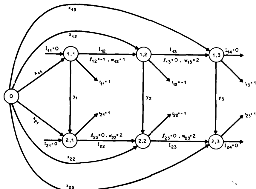
FIGURE 4. A network flow representation of the example
