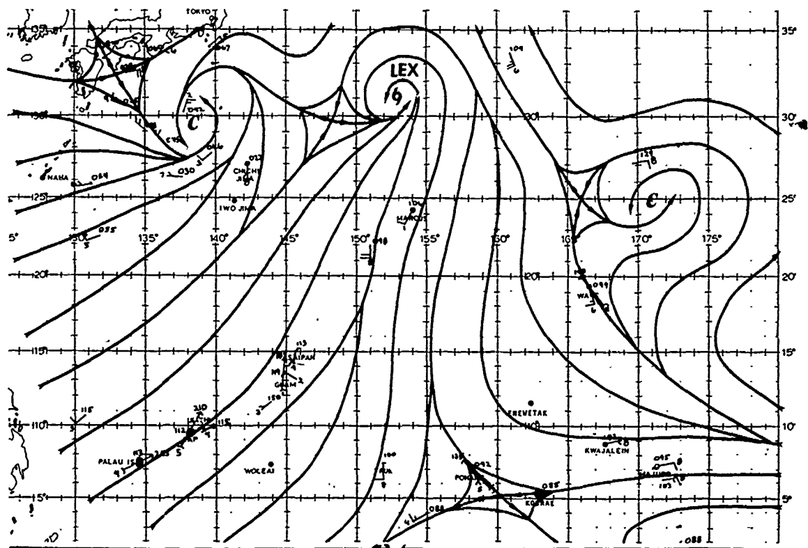
FIGURE 3-13-1. The 051200Z August 1980 surface 1/gradient-level (ddd) wind data and streamline analysis. Wind speeds are in knots.
