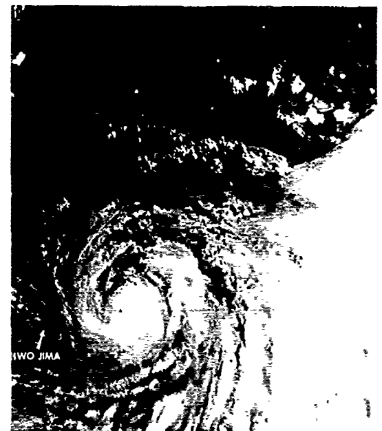
FIGURE 3-12-2. Typhoon Lex at maximum intensity of 80 kt (41 m/sec), 2 August 1980, 2242Z. Iwo Jima is about 155 nm (285 km) west of Lex. (NOAA6 imagery)
