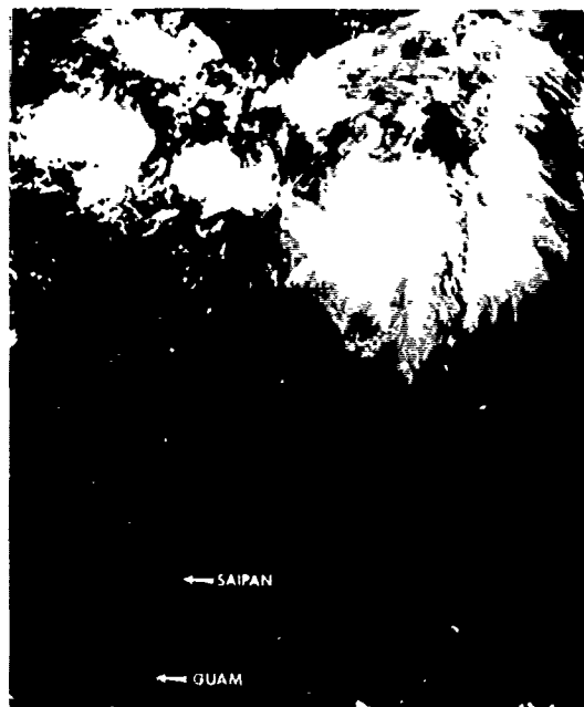
FIGURE 3-12-1. Lex as a tropical disturbance prior to issuance of a TCFA, 27 July 1980, 0026Z. (DMSP imagery)
