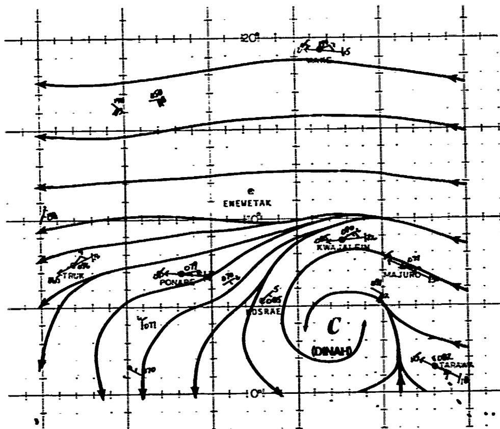
FIGURE 3-27-1. The 200000Z November 1980 surface (—) / gradient-level (---) wind data and streamline analysis. Wind speeds are in knots.
