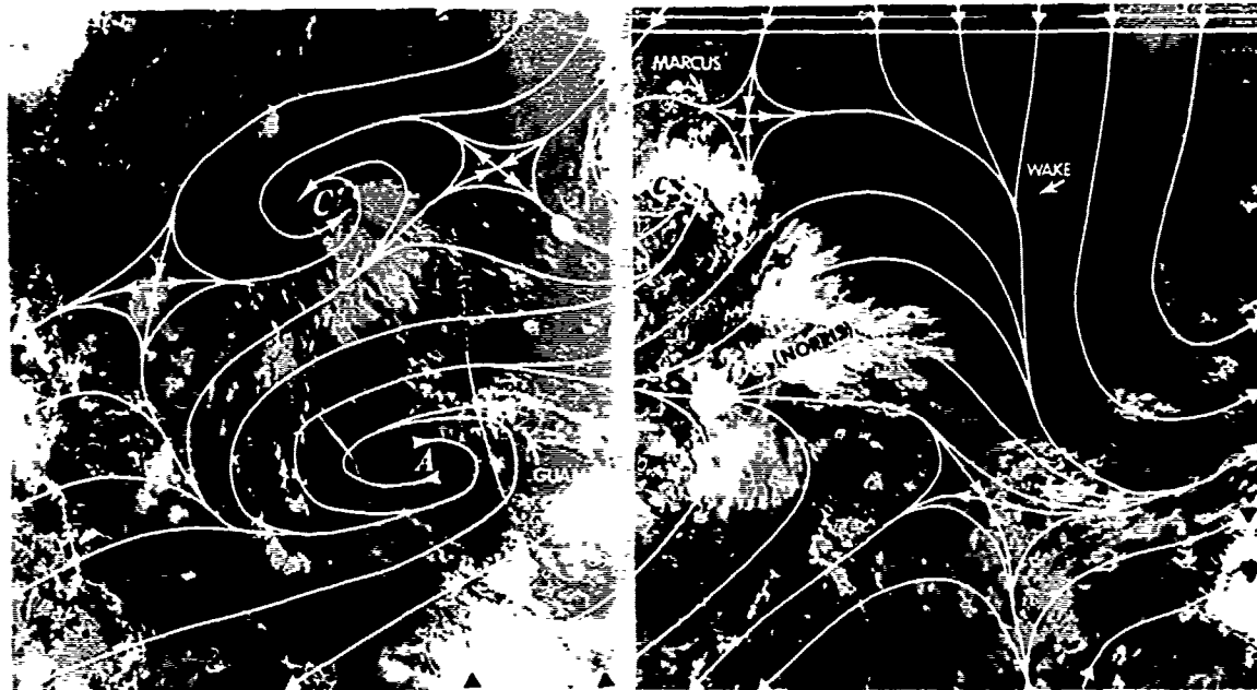
FIGURE 3-15-1. 210000Z August 1980 200 mb streamline analysis superimposed on satellite imagery at 202200Z. This figure depicts convective activity associated with upper-level cyclonic circulations and the enhanced convection southeast of the TUTT that eventually developed into Typhoon Norris. (NOAA6 imagery)
