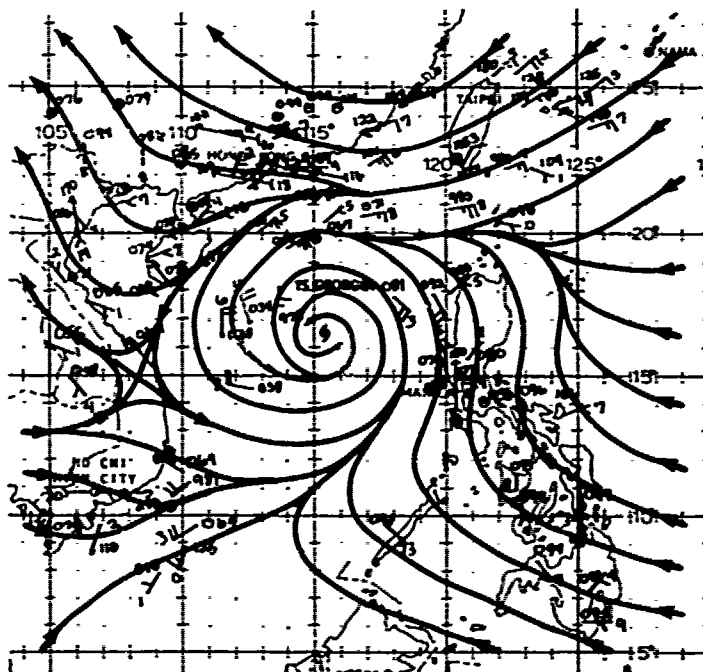
FIGURE 3-06-3. The 220000Z May 1980 surface level stream-line analysis in the vicinity of Tropical Storm Georgia. Winds are in knots.
