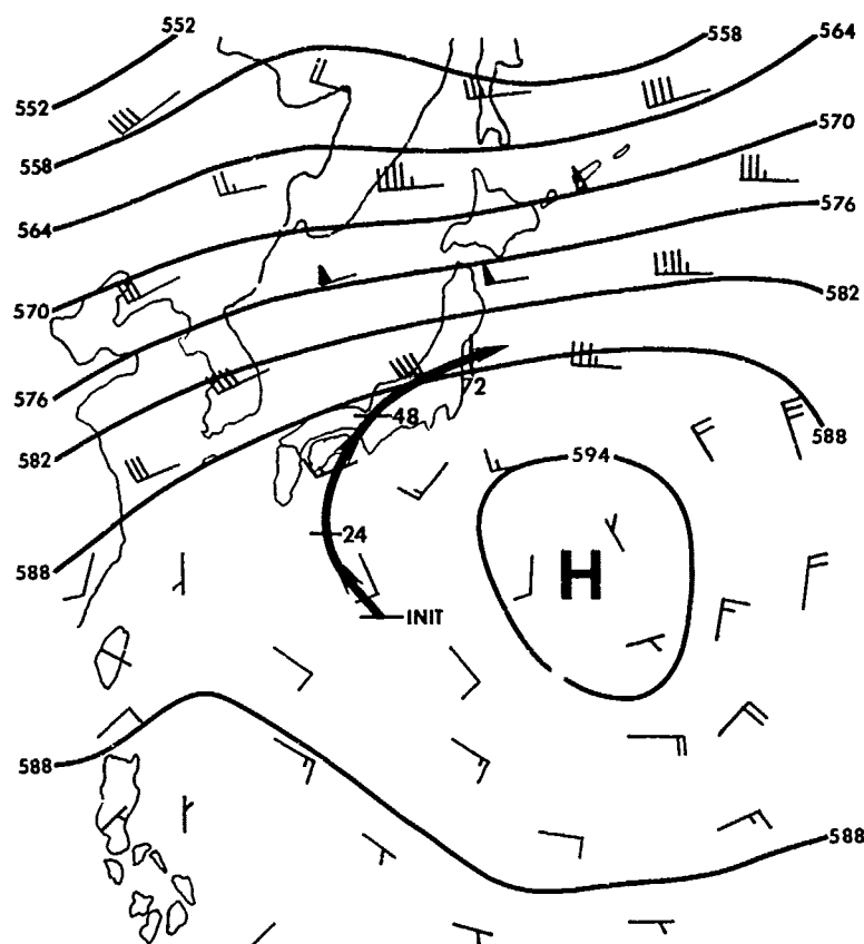
FIGURE 3-20-4. The 48 hour 500 mb numerical forecast chart based on the 161200Z September computer analysis. JTWC's 170000Z September forecast track for Sperry is also indicated, from initial position to the 72 hour forecast position.
