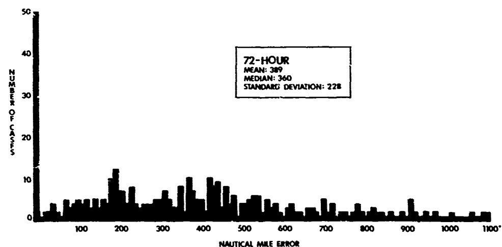
FIGURE 4-1. Frequency distribution of 1979 24-, 48-, and 72-hour forecast vector errors for all significant tropical cyclones in the western North Pacific.
