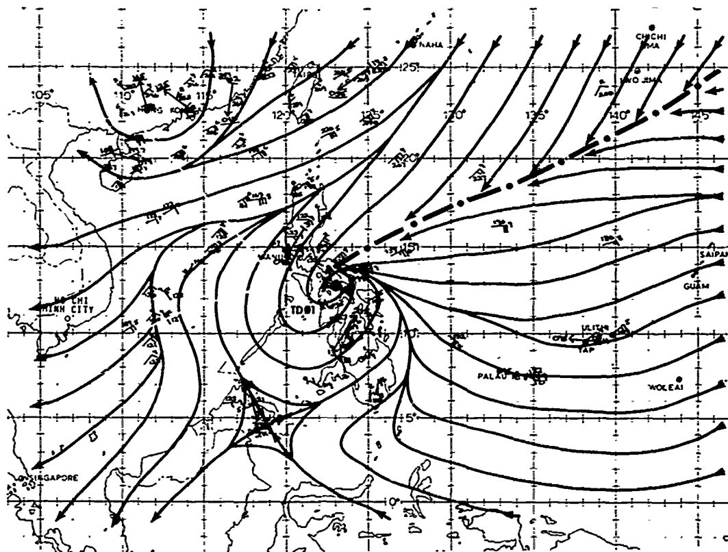
FIGURE 3-01-2. The 240000Z March 1980 surface (---) / gradient-level (ddd---<46) wind data and streamline analysis. Wind speeds are in knots.
