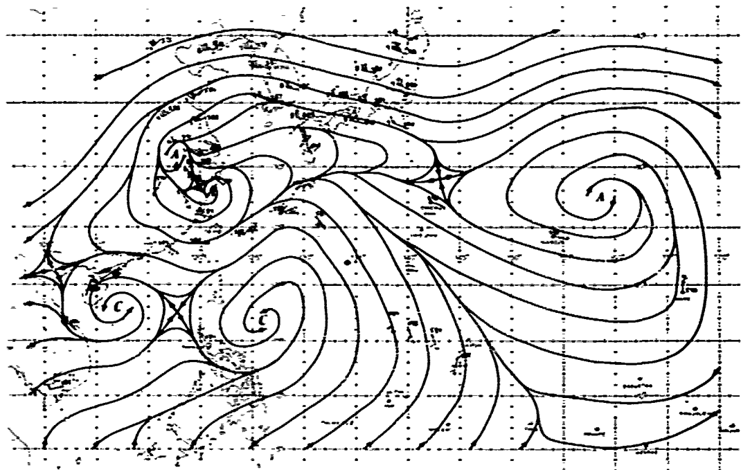
FIGURE 3-20-1. The 141200Z September 1950 500 mb streamline analysis. Wind speeds are in knots.
