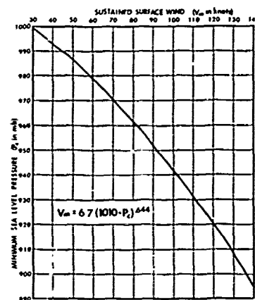
FIGURE 3-05-2. Atkinson and Holliday (1977) maximum sustained surface wind-minimum sea-level pressure relationship.
