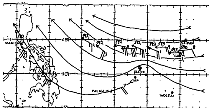
FIGURE 3-05-1. The 220000Z May 1980 streamline analysis of 500 mb rawinsonde (—) and aircraft reconnaissance (---) data. The 500 mb heights are plotted in decameters and wind speeds are in knots.
