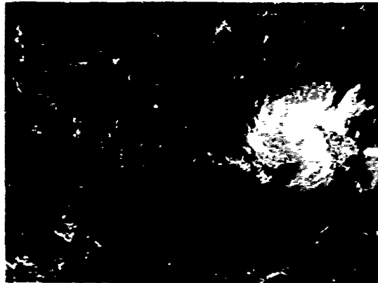
FIGURE 3-01-1. TD 01 at 15-20 kt (8-10 m/sec) intensity about 500 nm (926 km) south-southwest of Guam, 18 March 1980, 0120Z. (DNIS imagery)
