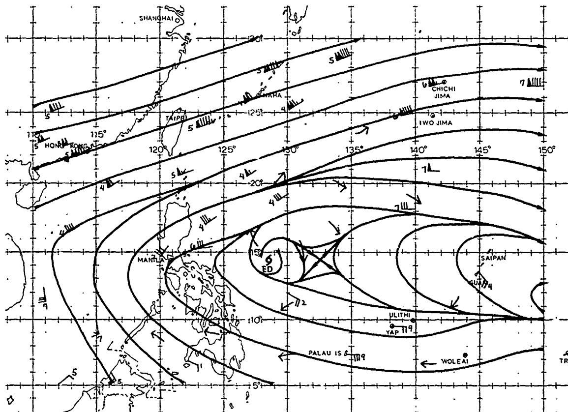
FIGURE 3-28-2. The 200000Z December 1980 200 mb streamline analysis. Wind speeds are in knots.
