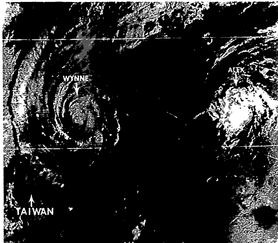
FIGURE 3-24-1. Visual imagery of Tropical Storm Alex at 30 kt (15 m/sec) intensity, 12 October 1980, 2314Z. (NOAA6 imagery)
