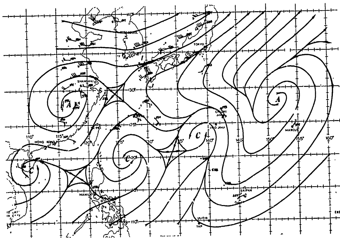
FIGURE 3-20-3. The 161200Z September 1980 500 mb streamline analysis. Wind speeds are in knots.
