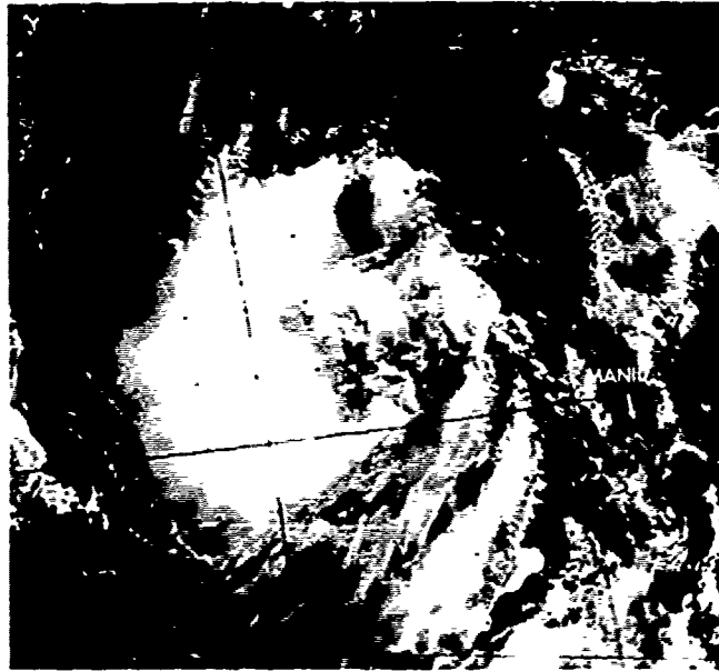
FIGURE 3-10-1. Tropical Depression 10 220 nm (407 km) west-northwest of Manila 13 hours prior to issuance of first warning. Heavy convection is located two degrees west of the surface circulation, 17 July 1980, 0203Z. (DMSP imagery)
