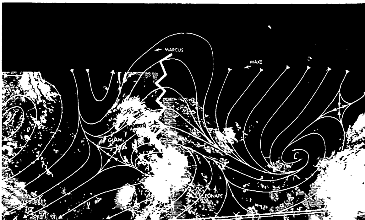
FIGURE 3-15-2. 220000Z August 1950 200 mb streamline analysis superimposed on satellite imagery at 212100Z. This figure illustrates convective heating which built a sharp ridge to the east of the TUTT cell. This ridge pushed the TUTT northward and eventually split it into two cells. (NOAA6 imagery)
