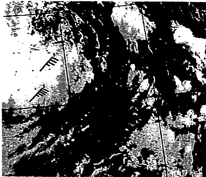
FIGURE 3-10-2. Tropical Depression 10 215 nm (398 km) south of Hong Kong with low-level circulation partially exposed due to strong vertical wind shear, 17 July 1980, 2334Z (NOAA6 imagery). Wind barbs represent aircraft and radiosonde reports near the 200 mb level at 171200Z.
