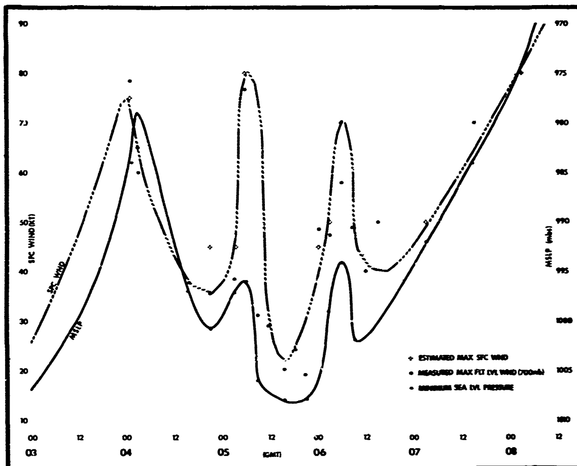
FIGURE 3-23-3. Smoothed traces of Myrre's maximum wind speed and minimum sea level pressure versus time for the period 3-9 October 1982.
