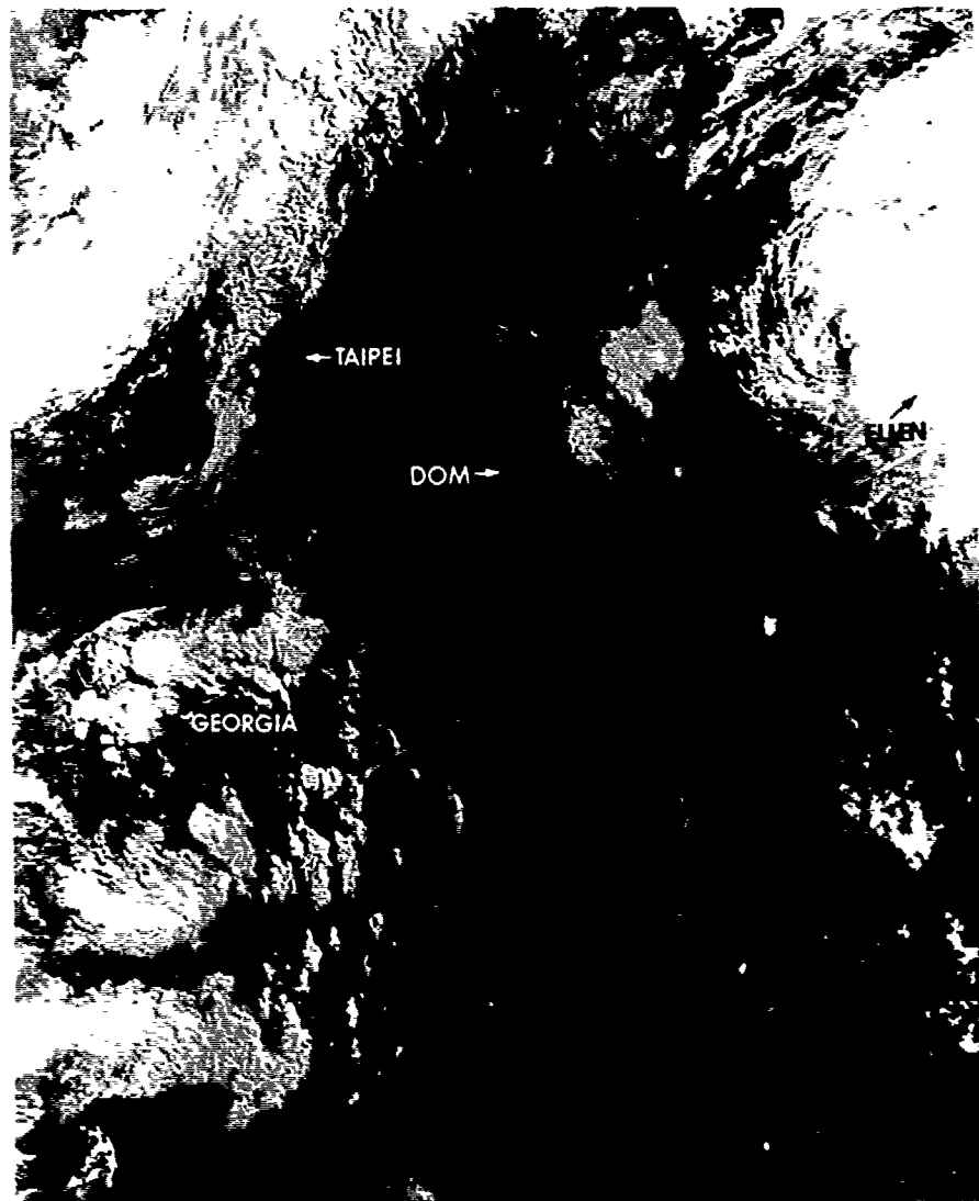
FIGURE 3-06-1. Typhoon Ellen, the remnants of Typhoon Dom, and the initial stage of Tropical Storm Georgia in the South China Sea, 19 May 1980, 2332Z. (NOAA6 imagery)
