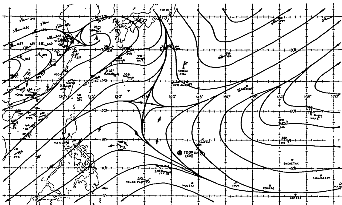
FIGURE 3-09-1. 200 mb streamline analysis at 171200Z July 1980. The analysis depicts the synoptic pattern which prevailed during much of Typhoon Joe's existence. Wind data are a combination of RAOBS, AIREPS, and satellite-derived (+) winds for the 250 mb to 150 mb levels. Wind speeds are in knots.
