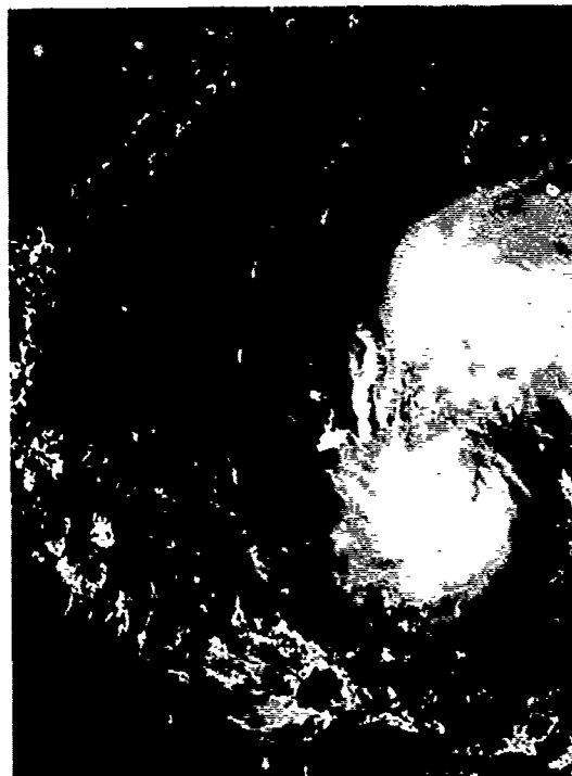
FIGURE 3-03-1. Typhoon Dom at 40 kt (21 m/sec) intensity tracking west-northwestward at 9 kt (17 km/hr), 11 May 1980, 0213Z. (DMSP visual imagery)
