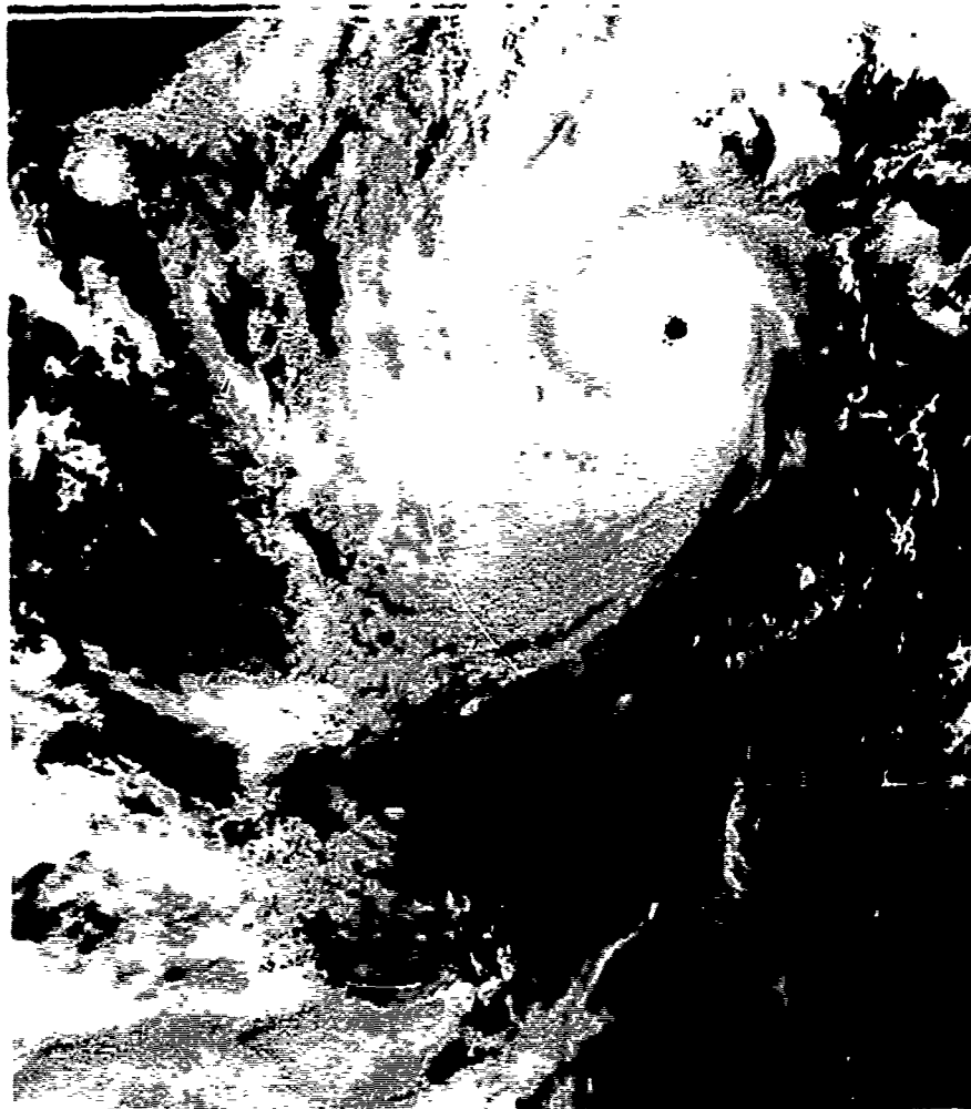
FIGURE 3-19-3. Typhoon Percy with 110 kt (57 m/sec) maximum surface winds while intensifying rapidly to near super typhoon strength, 17 September 1980, 0645Z. (Tiro's 4 imagery)
