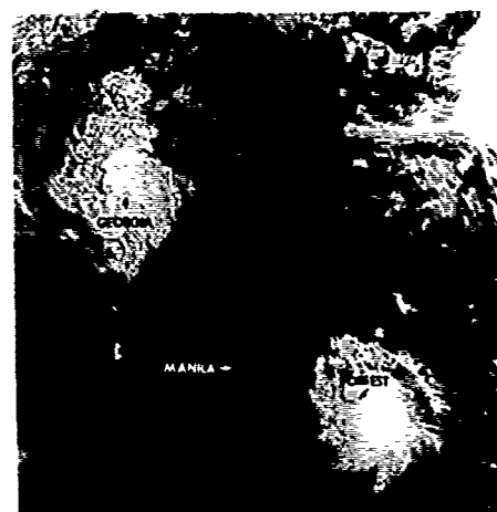
FIGURE 3-05-3. Tropical Storm Forrest at maximum intensity, 23 May 1980, 2344Z. Tropical Storm Georgia is making landfall over southeastern China. (NOAA 6 imagery)
