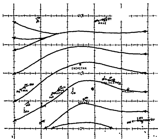
FIGURE 3-27-2. The 201200Z November 1980 surface (1/gradient-level (ddd) (6)) wind data and streamline analysis. Wind speeds are in knots. (●) indicates satellite position of Dinah at about the same time.
