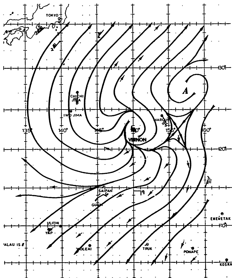
FIGURE 3-22-2. Upper-level streamline analysis (near the 200 mb level) at 011200Z October 1980. Data are rawinsonde and aircraft winds (—) and satellite-derived wind vectors (→). Winds are in knots.
