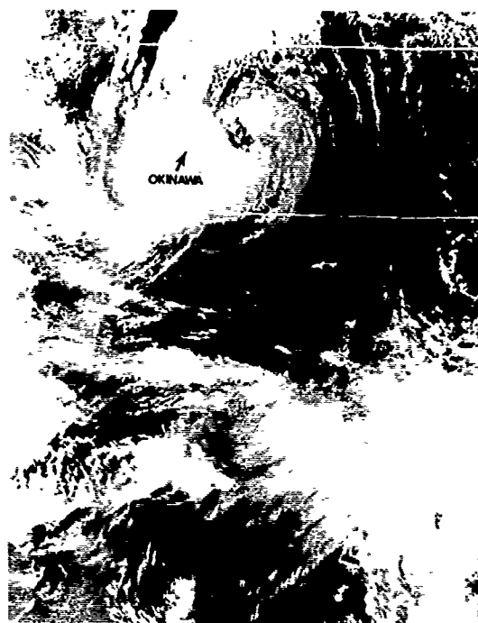
FIGURE 3-17-3. Typhoon Orchid, near maximum intensity, completing the second of three cyclonic loops, 10 September 1980, 0625Z. (TIROS-N imagery)
