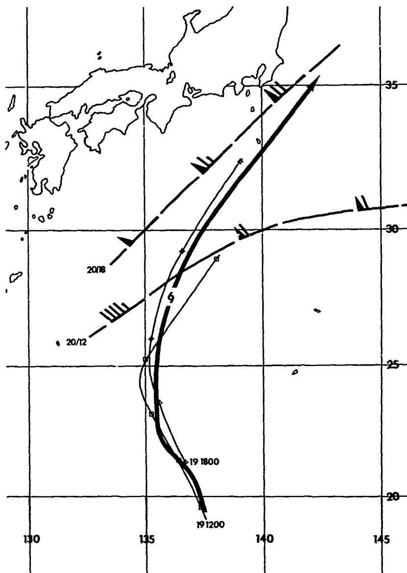
FIGURE 3-04-3. Forecast tracks for Typhoon Ellen from 191200Z and 191800Z data bases. Selected 24-hr forecast wind vectors at 500 mb for each data base are also illustrated, along with the final best track (—) for that period.
