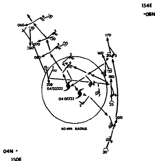
FIGURE 3-23-1. Plot of aircraft reconnaissance data for the 040122Z and 040332Z October 1950 fixes of Tropical Storm Wynne.
