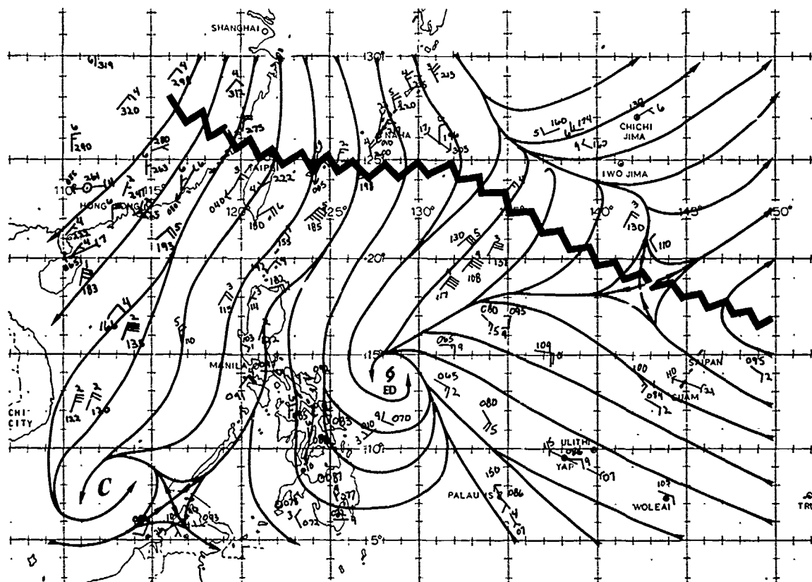
FIGURE 3-28-1. The 200000Z December 1980 surface (—) / gradient level (—) wind data and stream-line analysis in the vicinity of Tropical Storm Ed. Wind speeds are in knots.
