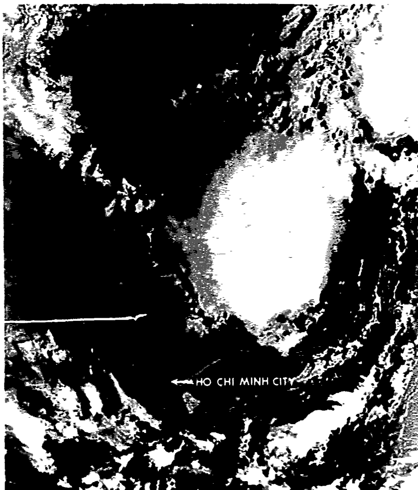
FIGURE 3-26-1. Tropical Storm Cary near maximum intensity in the South China Sea. The surface center is partially exposed as indicated by the cumulus banding southeast of the main convection, 01 November 1980, 0033Z. (NOAA6 imagery)
