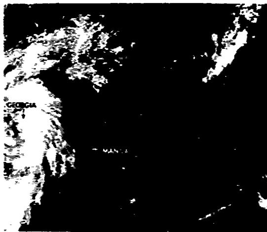
FIGURE 3-06-4. Tropical Storm Georgia at 45 kt (23 m/sec) intensity, 22 May 1980, 0150Z. (DMSP imagery)
