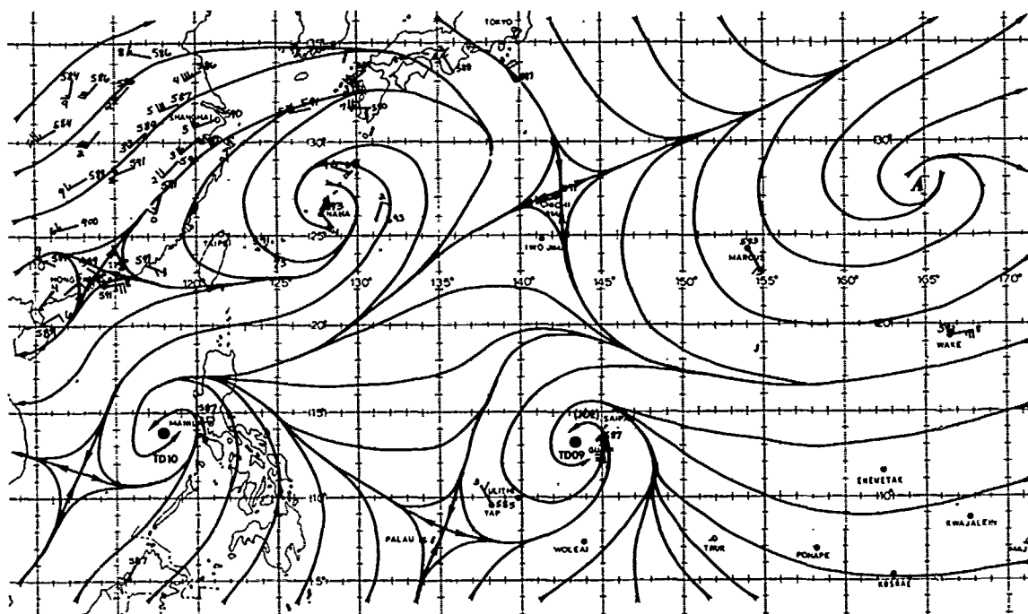
Figure 3-09-2. 500 mb streamline analysis at 170000Z July 1980. The analysis depicts the synoptic pattern which prevailed during much of Typhoon Joe's existence. Wind speeds are in knots.
