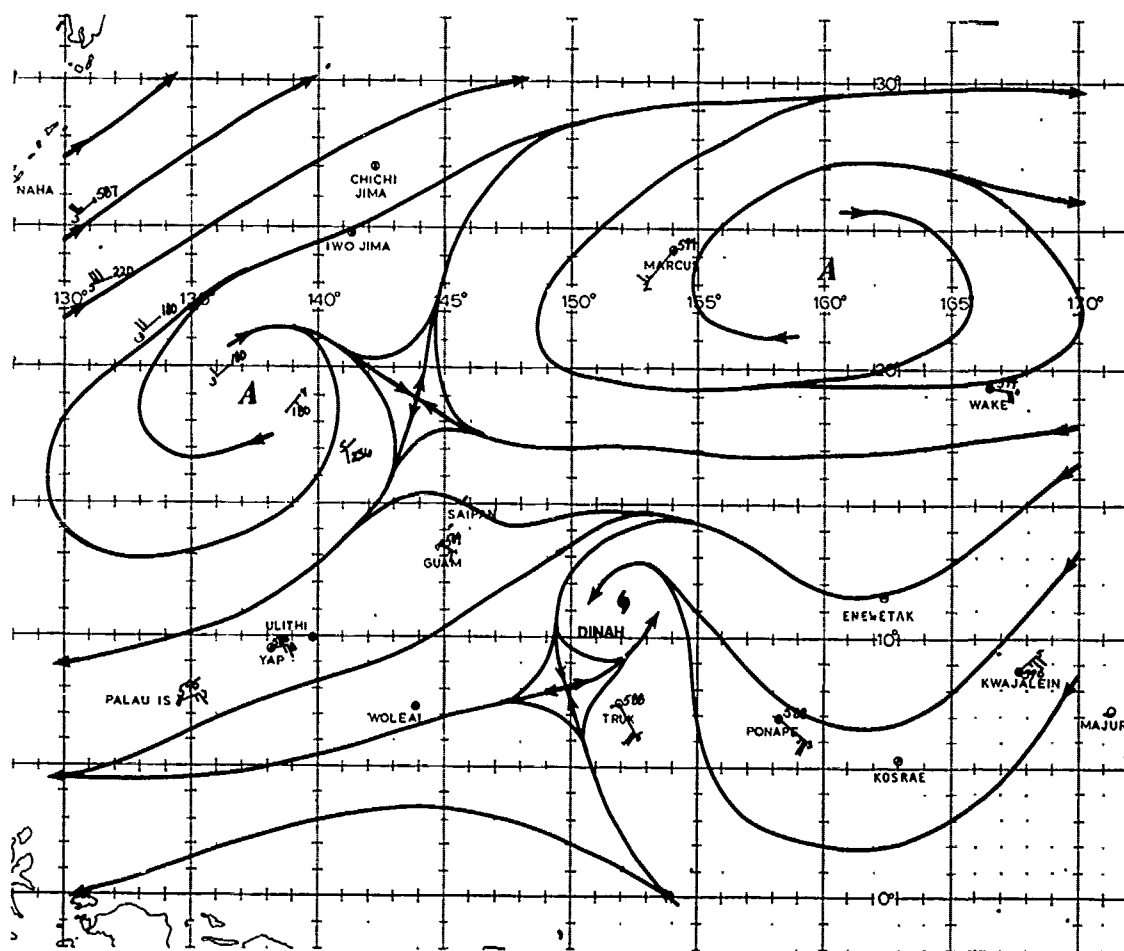
FIGURE 3-27-4. The 220000Z November 1980 500 mb wind data and streamline analysis. Wind speeds are in knots. Note the AIREPS northwest of Guam which were provided to JTWC by a Navy aircraft evacuating from Guam to Okinawa.
