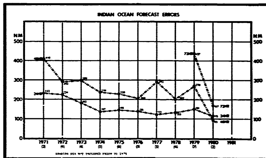
FIGURE 4-5. Annual mean vector errors (nm) for all cyclones in the north Indian Ocean.
