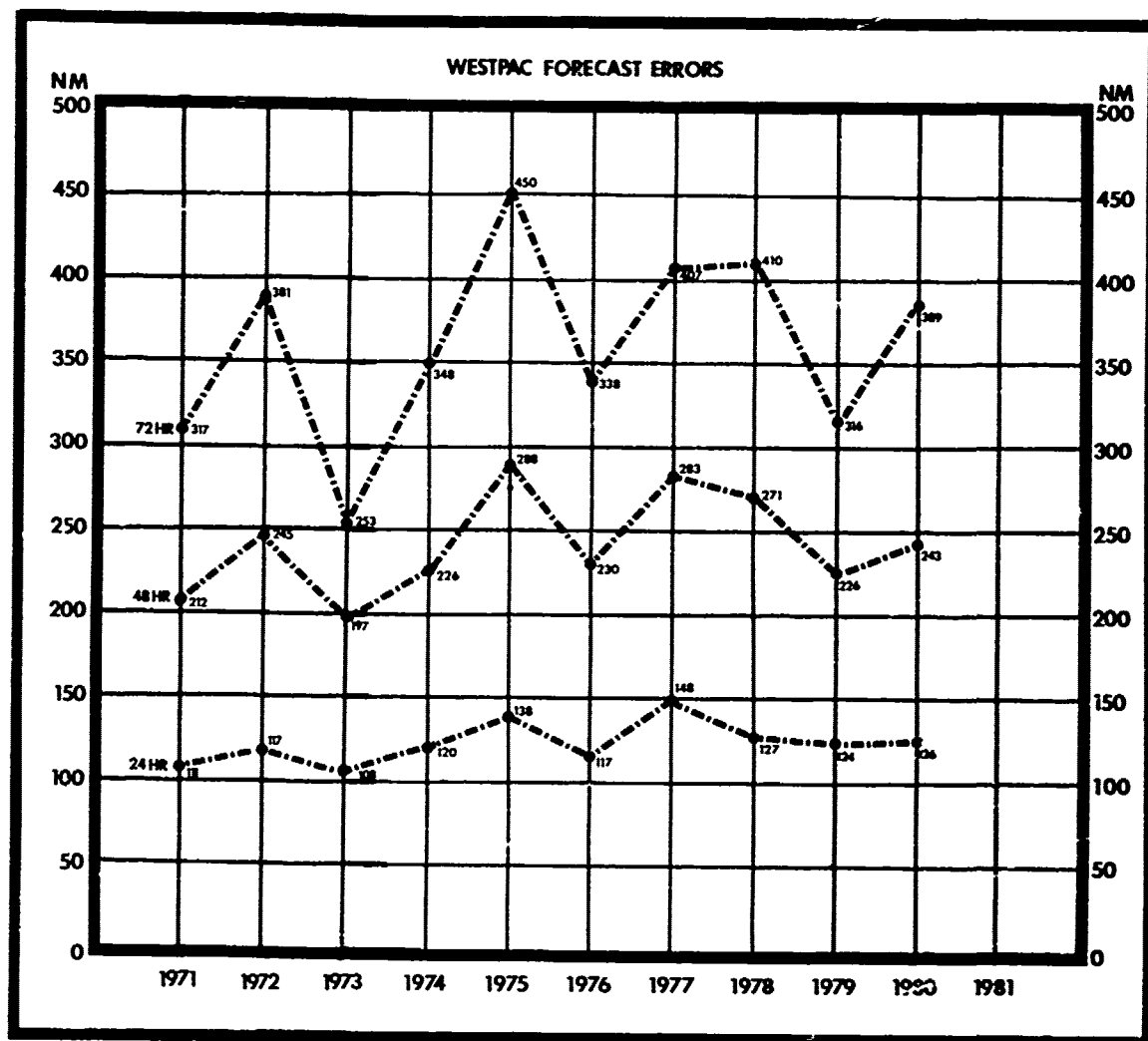
FIGURE 4-2. Annual vector errors (nm) for all cyclones in the western North Pacific.
