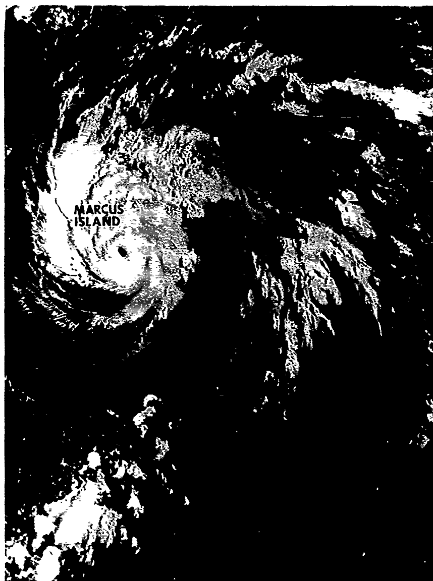
FIGURE 3-13-5. Visual satellite imagery of Typhoon Marge just after reaching maximum intensity and minimum sea-level pressure, 10 August 1980, 2124Z. (NOAA6 imagery)
