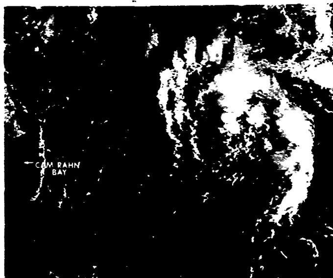
FIGURE 3-01-3. The remnant of TD 01 in the South China Sea showing signs of regeneration, 26 March 1980, 0206Z. (DMSP imagery)
