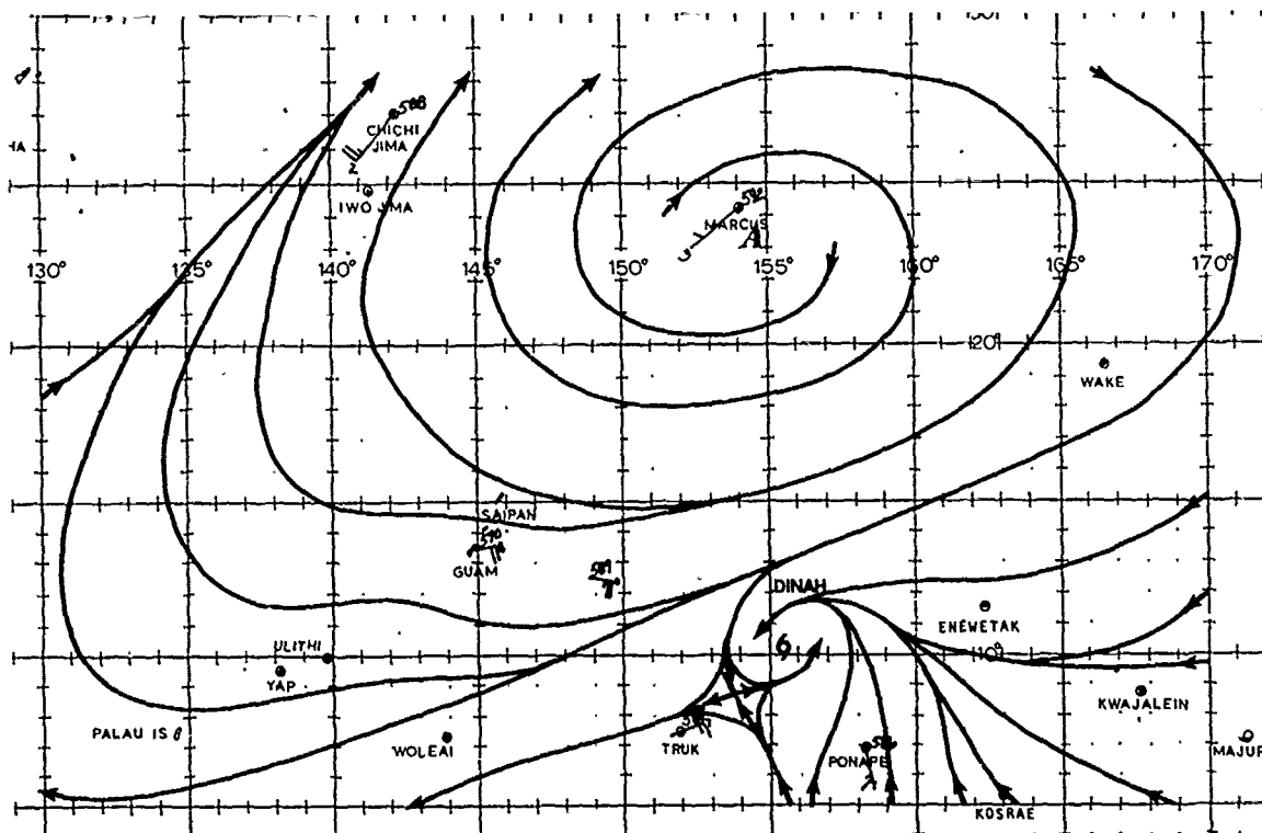
FIGURE 3-27-3. The 211200Z November 1980 500 mb wind data and streamline analysis. Wind speeds are in knots.
