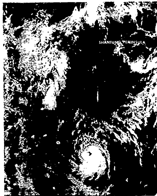
FIGURE 3-07-1. Tropical Storm Herbert at 45 kt (23 m/sec) intensity making landfall over southern China, 28 June 1980, 0316Z. (DMSP imagery)
