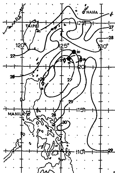
FIGURE 3-03-3. Composite sea surface temperature analysis of data from 17-23 May 1980, produced by the Oceanographic Services Division of Naval Oceanography Command Center, Guam.
