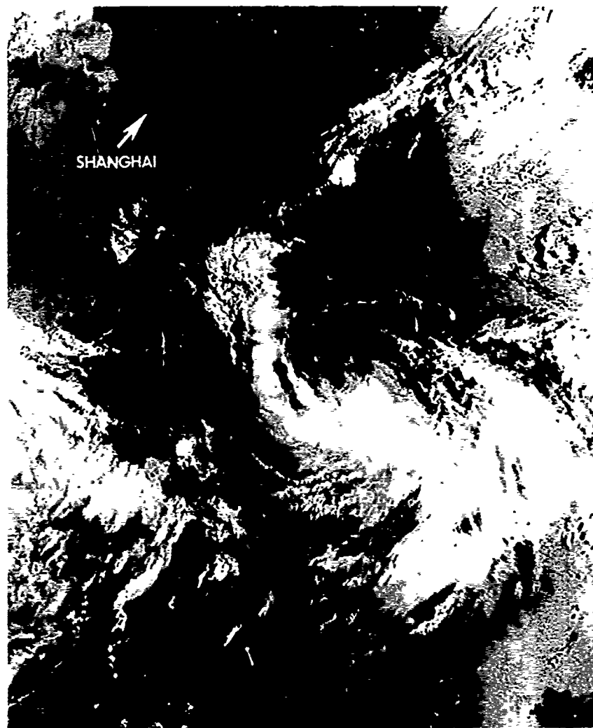
FIGURE 3-19-1. Tropical Storm Percy at 45 kt (23 m/sec) intensity, 14 September 1980, 2333z. Percy's low-level center at that time was partially exposed on the northeastern edge of a large convective area. (NGAA6 imagery)
