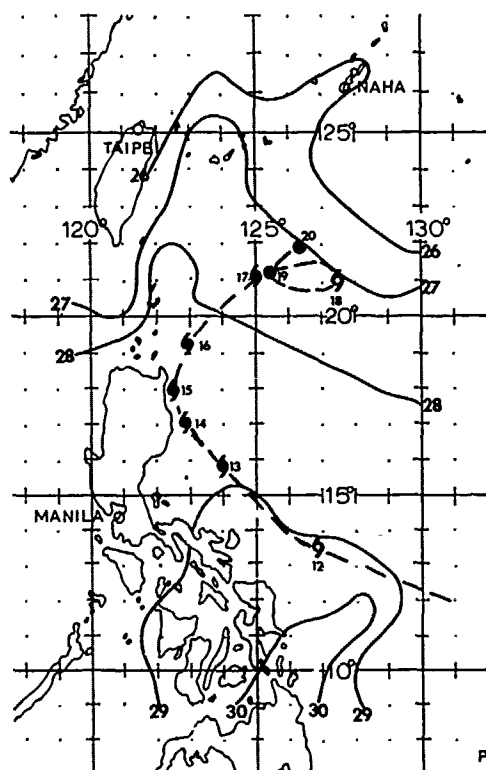
FIGURE 3-03-2. Composite sea surface temperature analysis of data from 10-16 May 1980, produced by the Oceanographic Services Division of Naval Oceanography Command Center, Guam.
