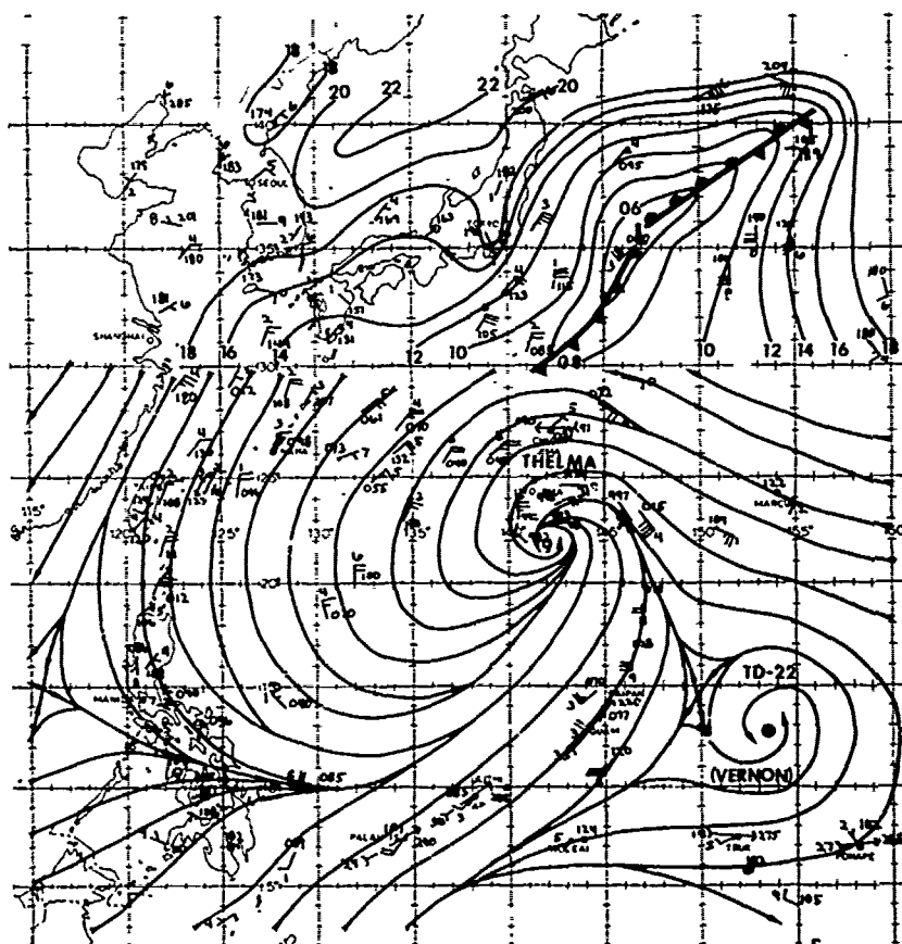
FIGURE 3-22-3. The 280000Z September 1980 surface 1/gradient-level (ddd<---<fff) wind data and streamline analysis. Winds speeds are in knots.
