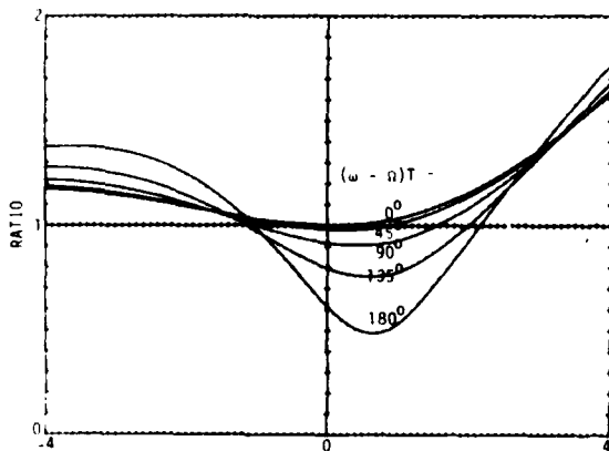
Figure 9. Amplitude Ratio for R-K(2,0.8)C.
