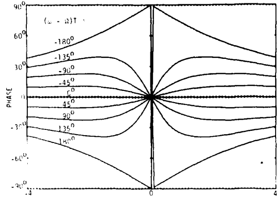
Figure 6. Phase Error for R-K(2,1)C.
