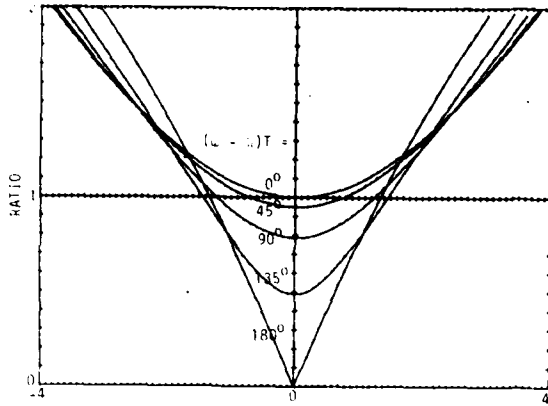
Figure 5. Amplitude Ratio for R-K(2,1)C.
