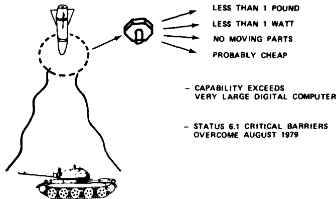
Figure 3. The simplest optical correlator seeker works on a top view.
