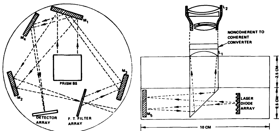
Figure 12. A Cylindrical coherent optical correlator.
