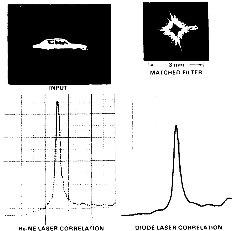
Figure 10. Performance of the Diode Laser Correlator
