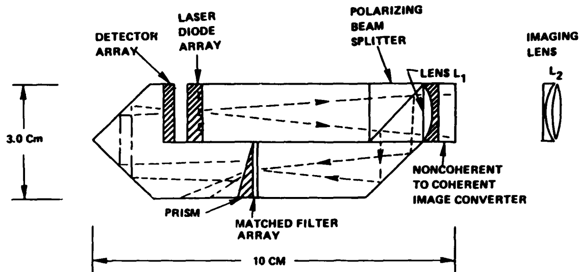
Figure 13. A Monolithic coherent optical correlator.
