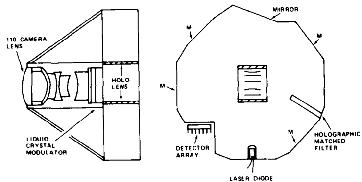
Figure 2. The optical correlator seeker in a visible mode.
