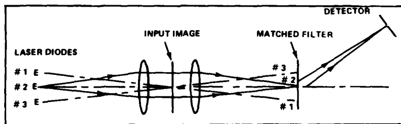
Figure 9. Multichannel optical correlator.
