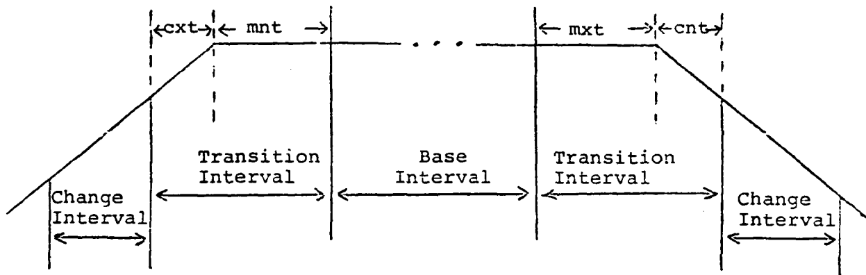
Figure 7. Definition of Transition Intervals.
