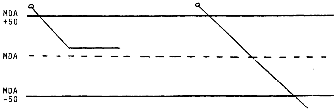
A. Stopping descent at the Minimum Descent Altitude
