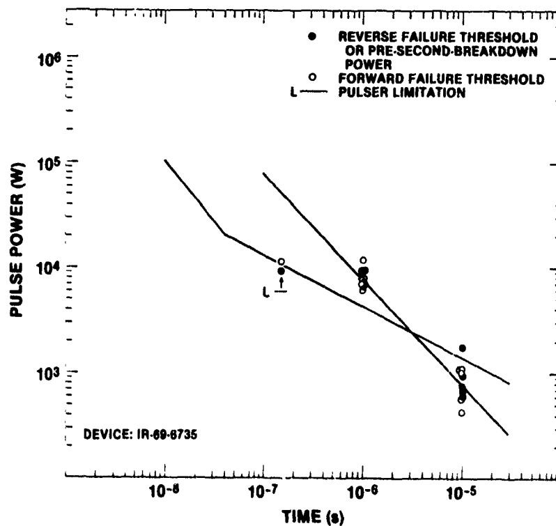
Figure A-14. Damage characteristics of IR-69-6735.
