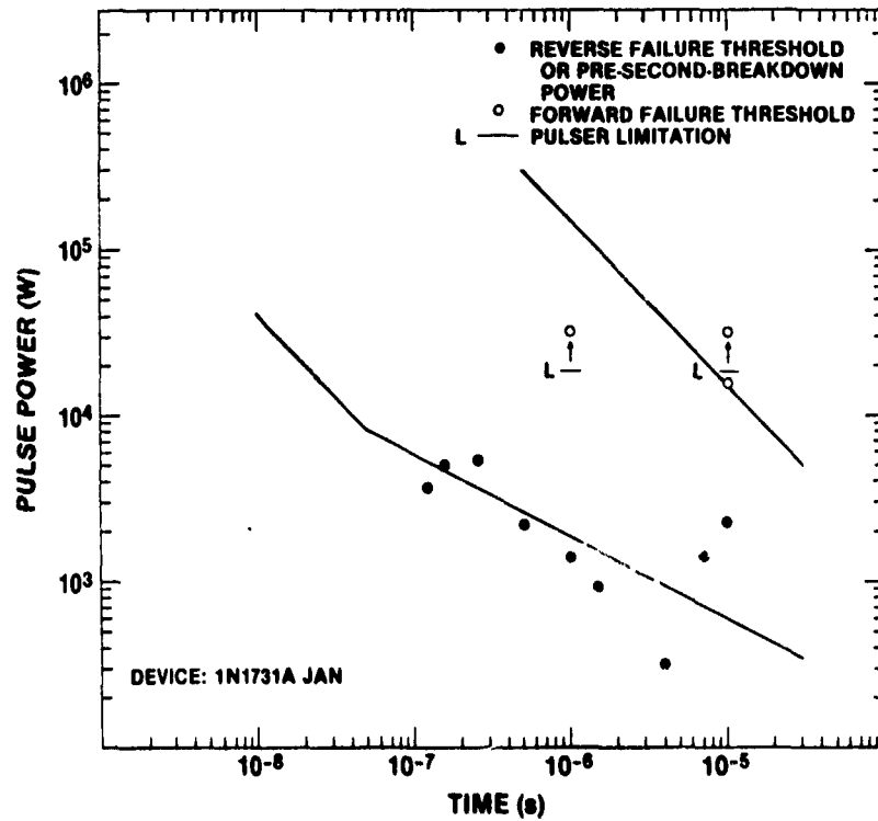
Figure A-9. Damage characteristics of 1N1731A JAN.
