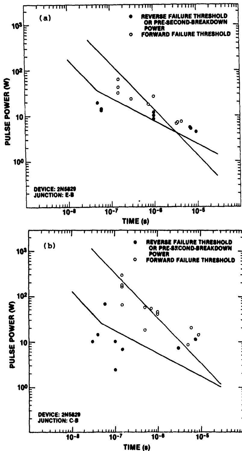
Figure A-37. Damage characteristics of 2N5829: (a) E-B junction and (b) C-B junction.
