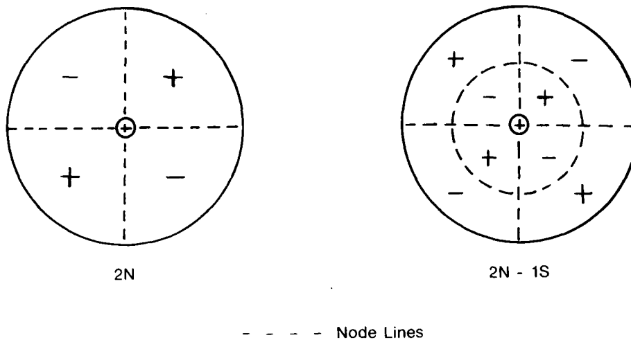
Figure 19. Typical Mode Shapes of 2N and 2N-1S Modes of Vibration of a Circular Disk
