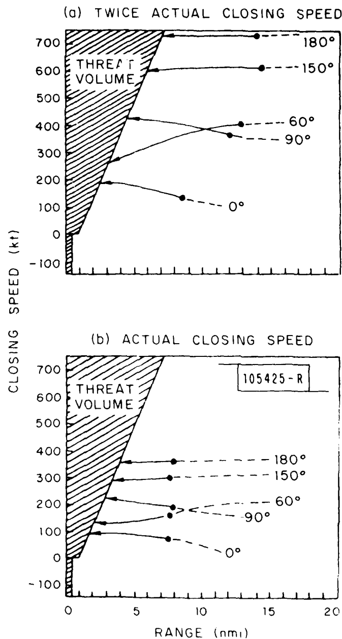
Fig. 3-9. Modified surveillance processor performance for five encounters.
