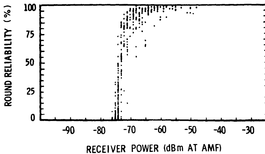
(a) BCAS Top-Antenna to Remitter Diversity
