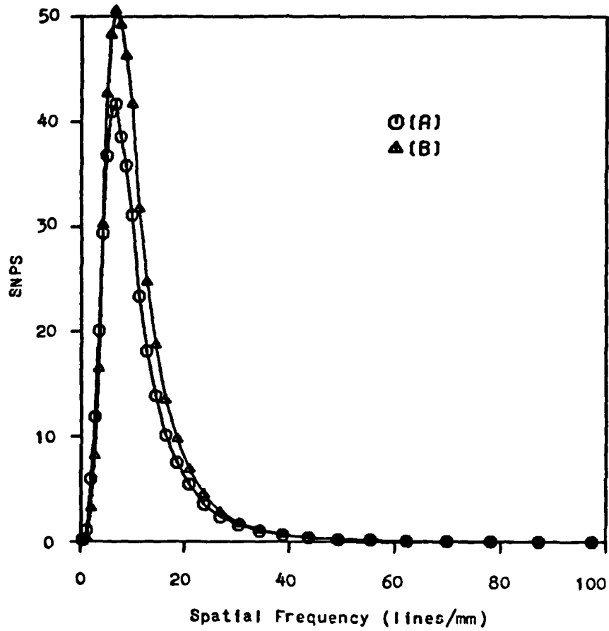
Fig. 4. SNPS of the random distribution of pebbles.
