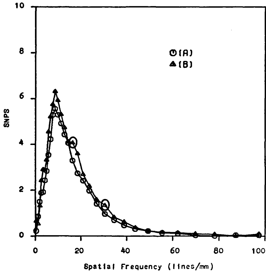
Fig. 13. Averaging effect of the coherent optical processor aperture for the random scene in Fig. 2D.
