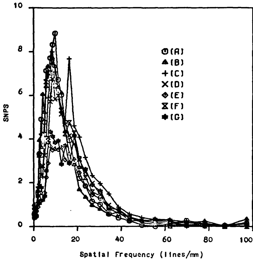
Fig. 10. Effect of aperture placement on the SNPS and information capacity of the random scene in Fig. 2D.
