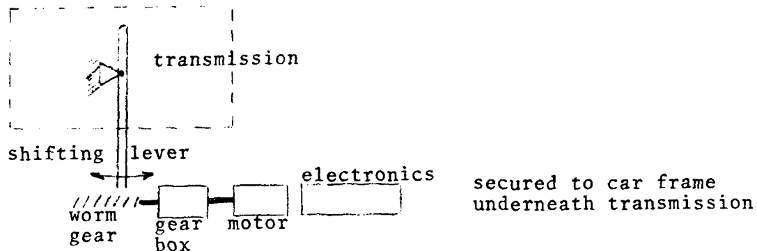
FIG 8 SHIFTING DRIVE MOTOR and ELECTRONICS
