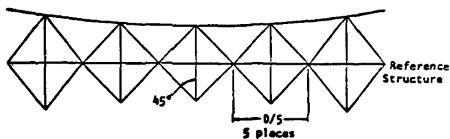
Fig. 5. Section view of truss configuration along meridional plane.
