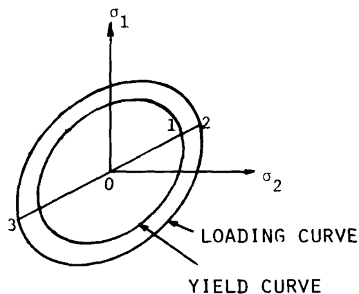
Figure 3. Isotropic Hardening
