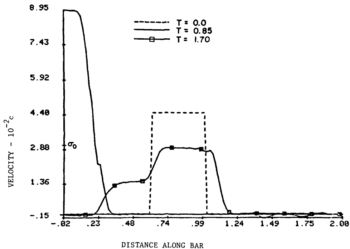
Fig. 6 Plastic Tensile Failure. v_0 = 1.5 \sigma_0
