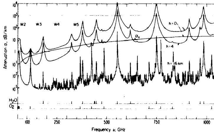
FIGURE 2. Attenuation rate \alpha at the altitudes, h = 0, 4, and 16 km over the frequency range, \nu = 100 GHz to 1000 GHz. The following atmospheric conditions and trace molecular number densities M(m^{-3}) were used in the calculation (24):
