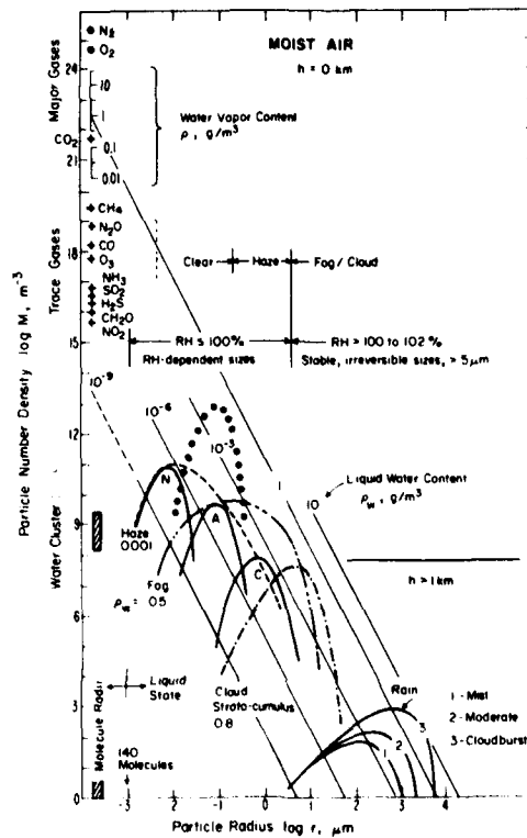
FIGURE 9. Schematic size distribution of number density M for equivalent spherical atmospheric particles from molecular to rain drop sizes, r = 10^{-4} to 10^4 \mu m (32,33,41).
