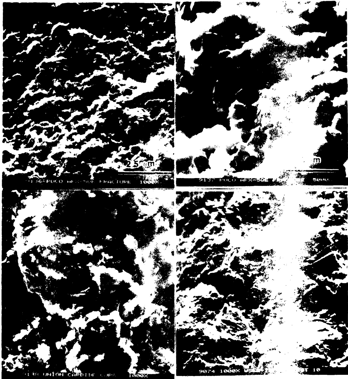
Figure 7 Fracture surface of 9127 Grade 90 Union Carbide C8000 (nickel aluminide) Westinghouse Corporation, Erie, Pa. Scanning Electron Micrograph.
