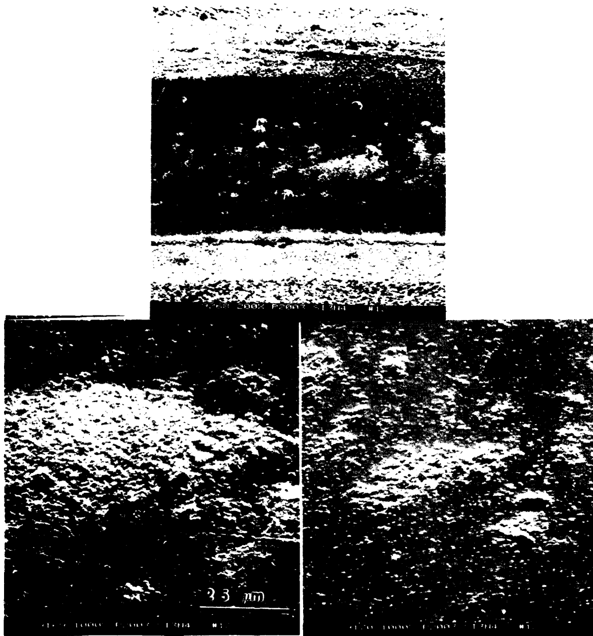
Figure 11 SEM photomicrograph of \text{Si}_3\text{N}_4 spindle ball wear track from Test 12. A Pure Carbon Co. P2003 graphite cage was used as the solid lubricant source. Test conditions: 1000°F (538°C) for 139 hours (187 million stress cycles).
