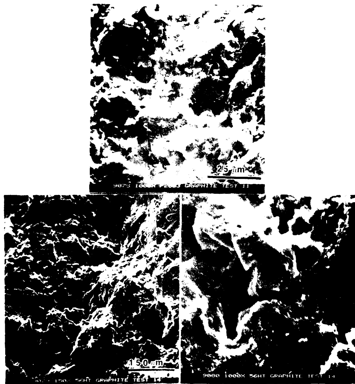
Figure 6 Fracture Surface of Graphite, 1000X and 50HT Grade Graphite, Electron Photomicrographs.
