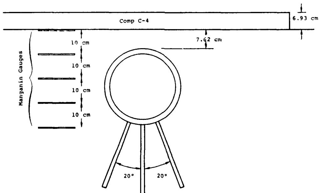
14(b) Schematic cross-section of test bed.
