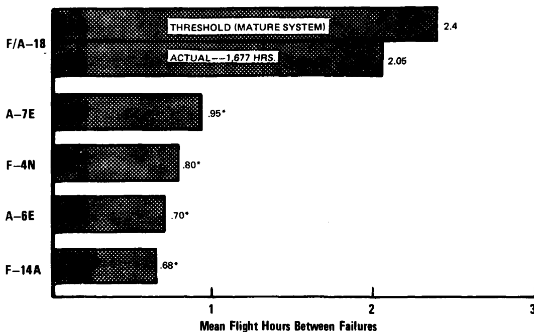
FIGURE 1 RELIABILITY COMPARISON
