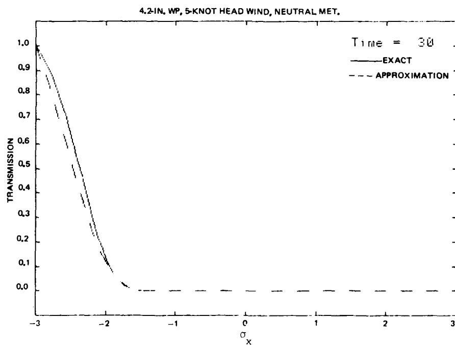
Figure 3. Comparison of transmission calculated using error function and Fermi function through smoke cloud at t = 30 .
