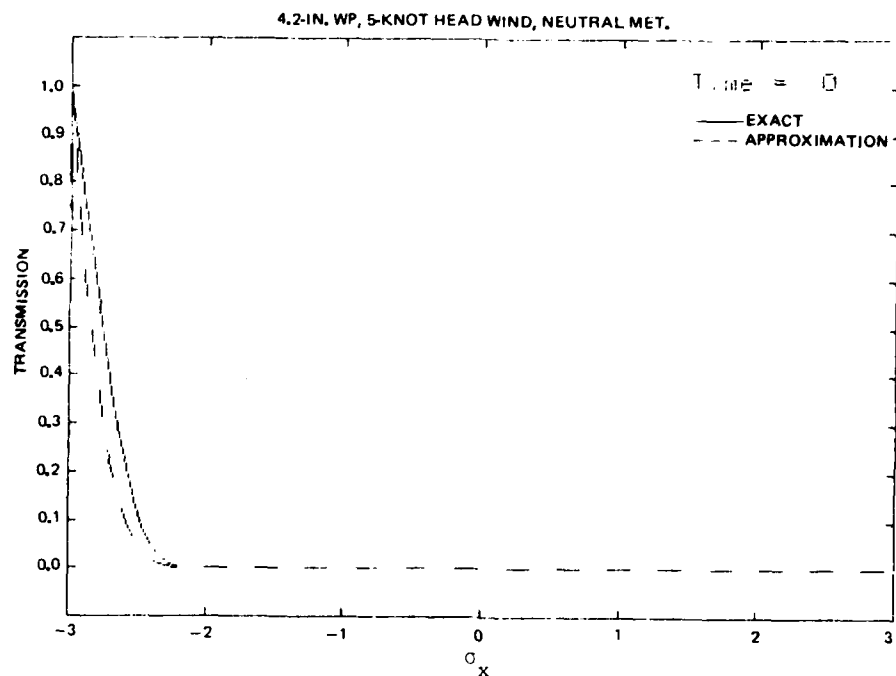
Figure 2. Comparison of transmission calculated using error function and Fermi function through smoke cloud at t = 0 .
