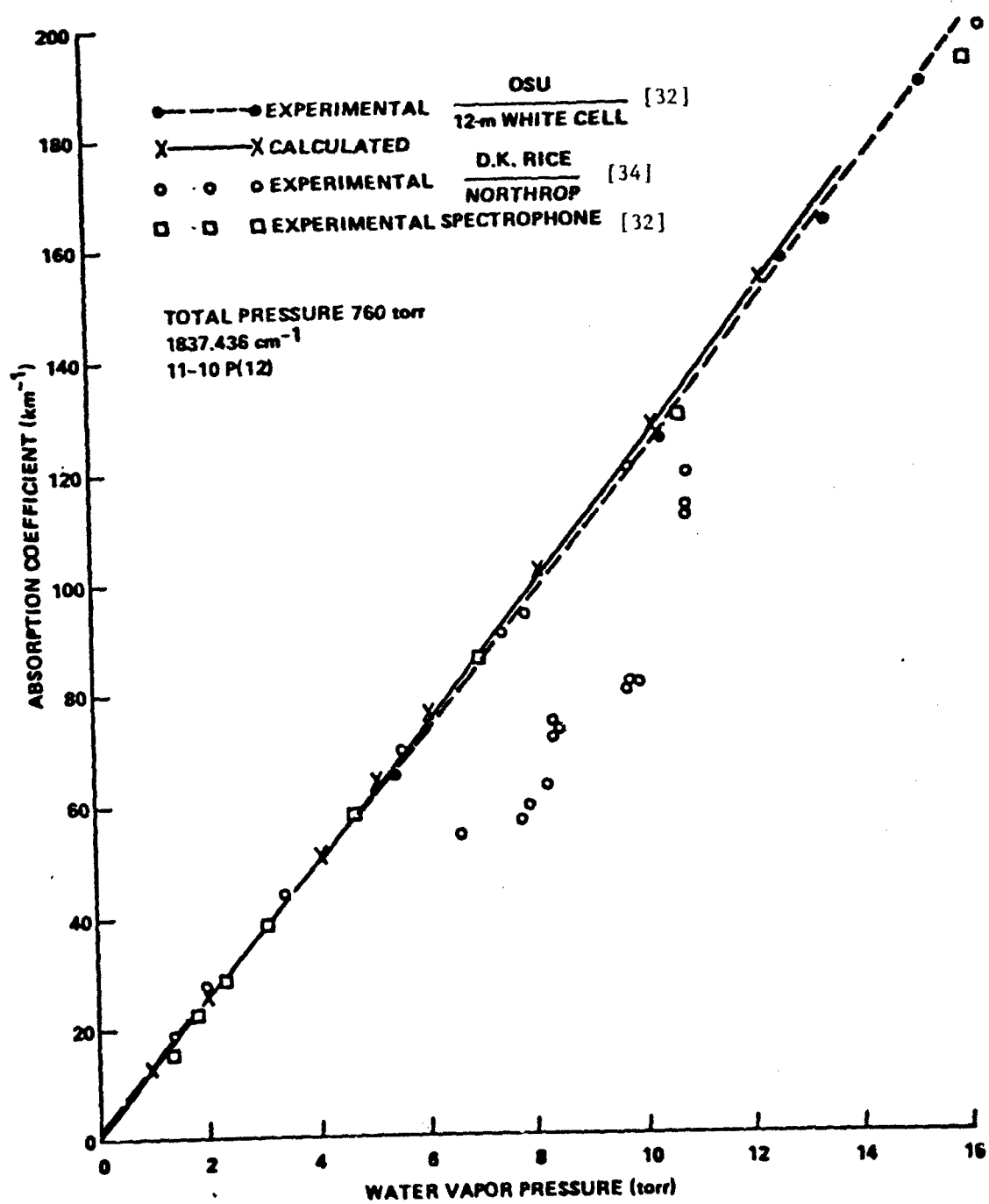
Figure 5. Measured and calculated data for water vapor absorption coefficient at 1837.436 \text{ cm}^{-1} [32].
