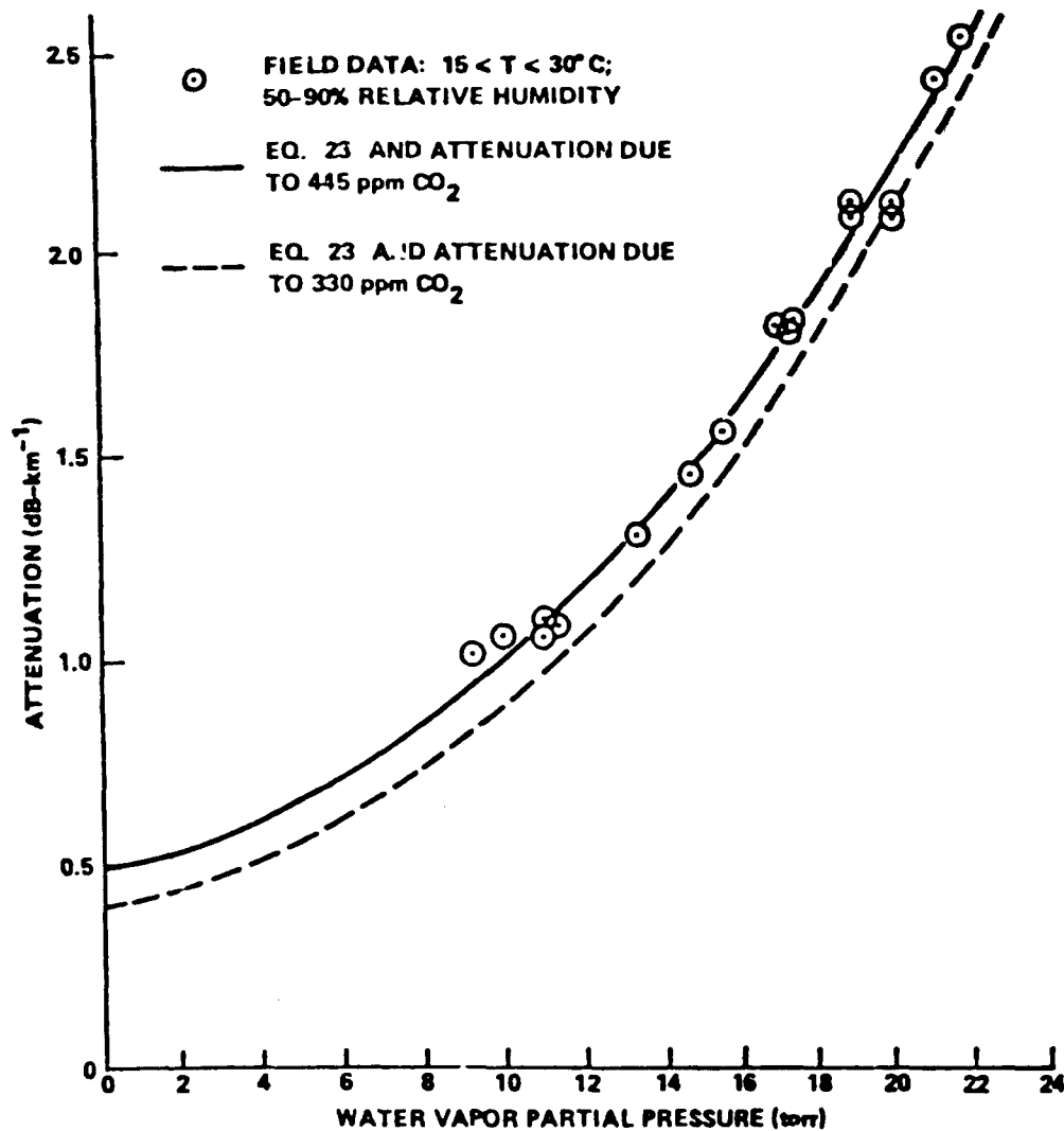
Figure 16. Field data of McCoy, et al. [13], at 10.59\text{ }\mu\text{m} compared with calculated attenuation based on Eq. 23 text.
