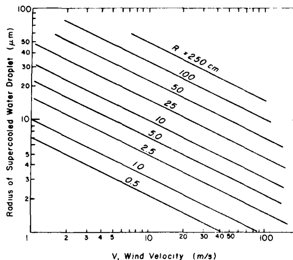
Figure 5. Critical radius of cylinder above which icing theoretically does not occur.
