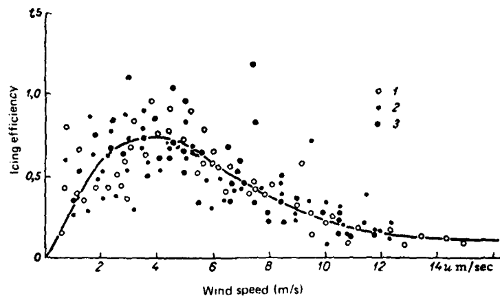
Figure 8. Dependence of icing efficiency (or capture coefficient) on wind speed for various liquid water contents w (Glukhov 1971), where 1) w = 0.12-0.16 \text{ g/m}^3 , 2) w = 0.17-0.21 \text{ g/m}^3 , 3) w = 0.22-0.26 \text{ g/m}^3 .
