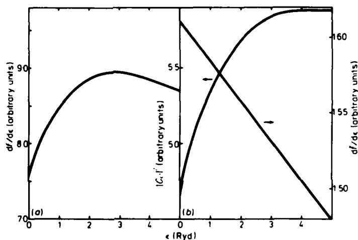
Figure 2. Cl K shell (a) df/d\epsilon ; (b) d\bar{f}/d\epsilon (right scale), |C_{e1}|^2 (left scale). See text for an explanation of these quantities.
