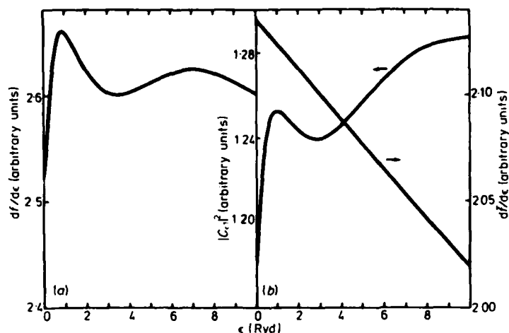
Figure 1. Cu K shell (a) df/d\epsilon ; (b) d\bar{f}/d\epsilon (right scale), |C_{e1}|^2 (left scale). See text for an explanation of these quantities.
