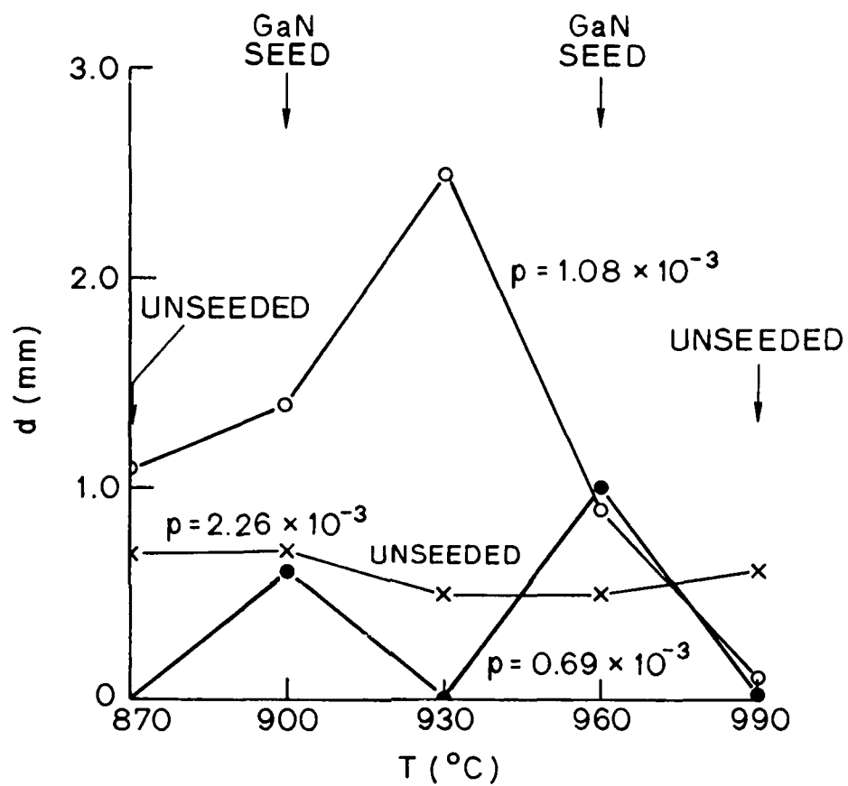
Fig. 8. Maximum crystal size versus temperature at various ammonia partial pressures.
