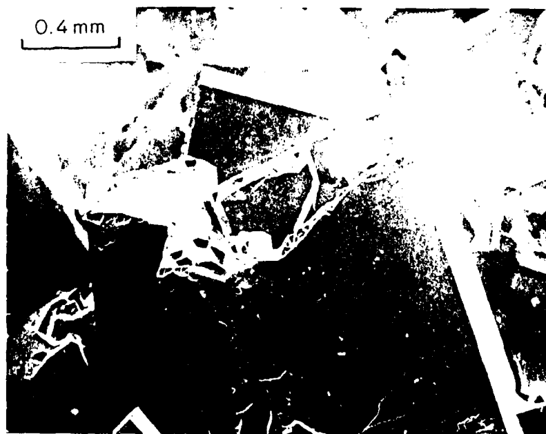
Fig. 15. (a) Cluster of hollow GaN crystals grown at 1.08 \times 10^{-2} partial pressure and 900^{\circ}\text{C} (20 X). (b) Magnified view of one hollow crystal (50 X).
