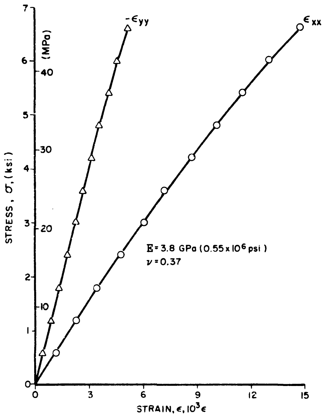
Figure 4 Stress-Strain Curves for DER 332 Epoxy Resin. Specimen No. 1-17 DB1 (Post-Cured at 367 degK, 200°F)
