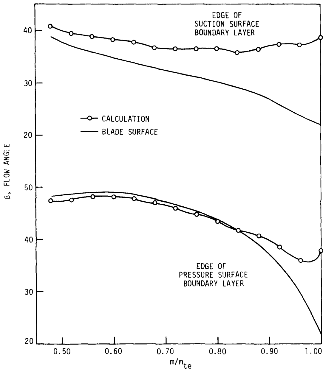
Figure 20. Calculated Flow Angle at the Edge of the Suction and Pressure Surface Boundary Layers for the NACA 65-(12)10 Blade Cascade. M_1 = 0.06 , Re_c = 1.47 \times 10^5 , \beta_1 = 57.7^\circ , \alpha = 12^\circ , D = 0.42 , \gamma = 45.7^\circ , \sigma = 1.0 , c = 124 mm, AVDR = 1.0
