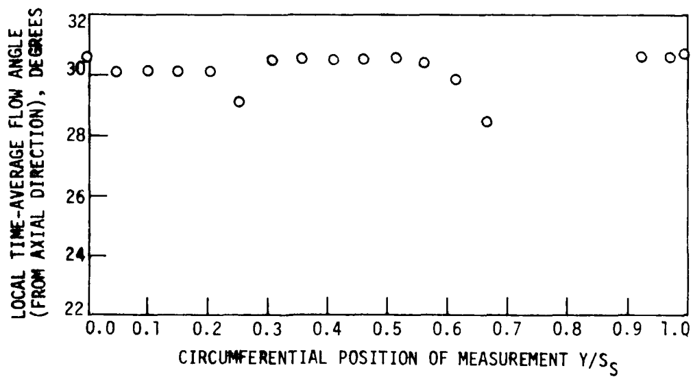
(b) Y0_{IGV}/S_S = 0 ; Y0_{1S}/S_S = 0.719
