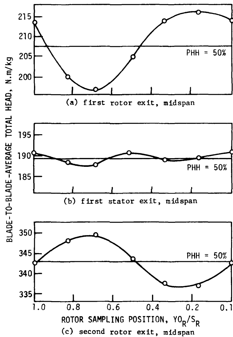
Figure. 17. Blade-to-blade-average total-head data.
