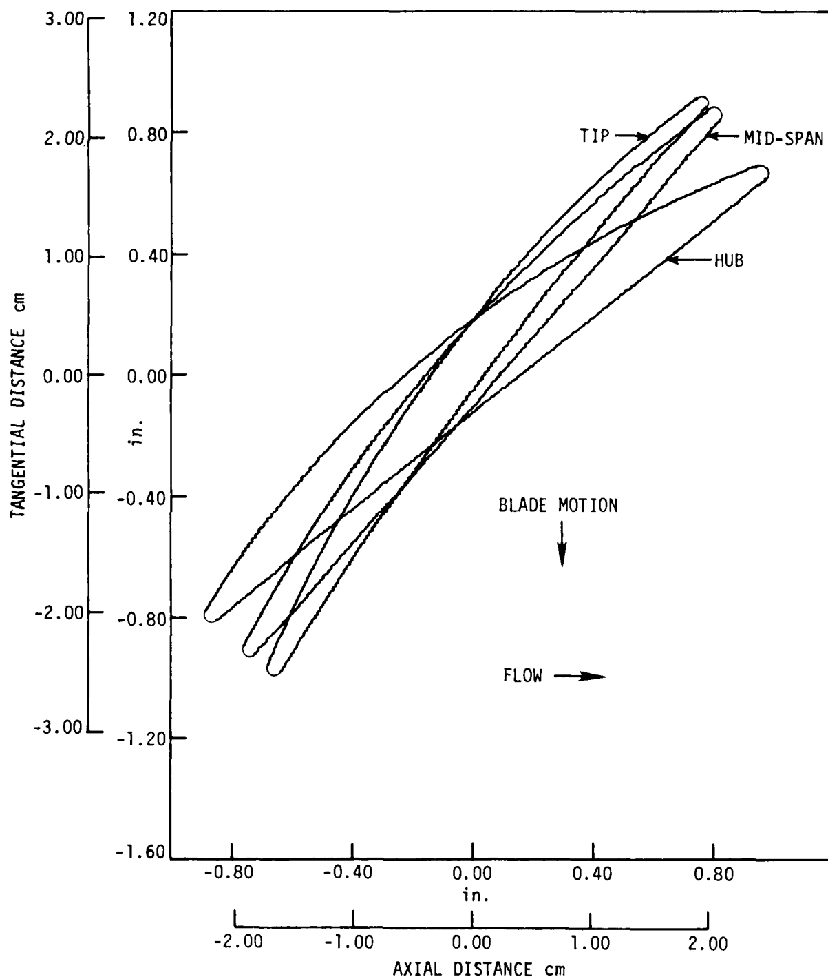
Figure 23. Representative baseline configuration rotor blade sections.
