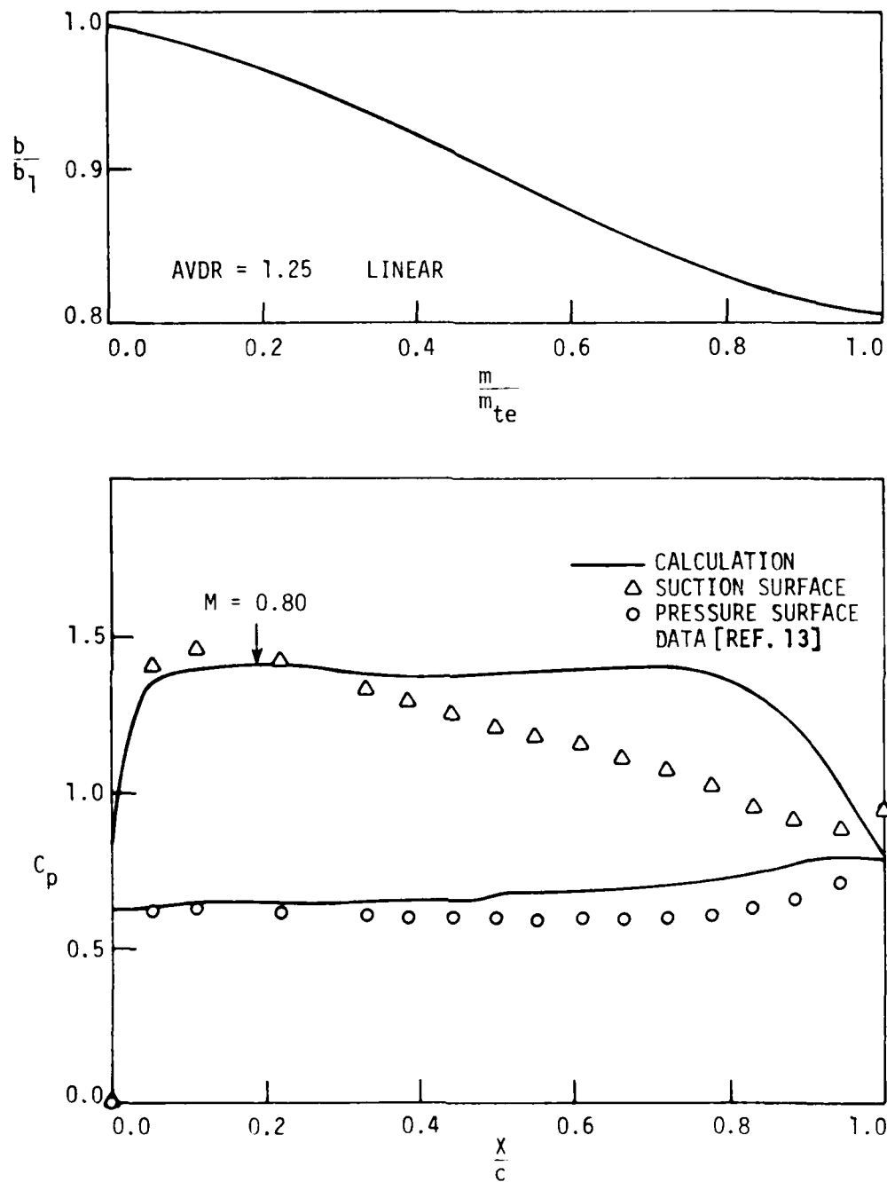
Figure 18. Calculated Surface Pressures Compared with Experimental Data for the DCA \phi = 48^\circ Blade Cascade.
