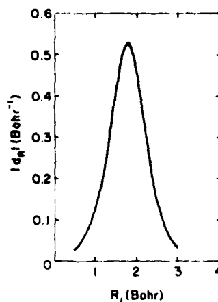
FIG. 2. The nonadiabatic coupling vs R_1 = R - \frac{1}{2}r , \lambda is assumed to be equal to 0.016.
