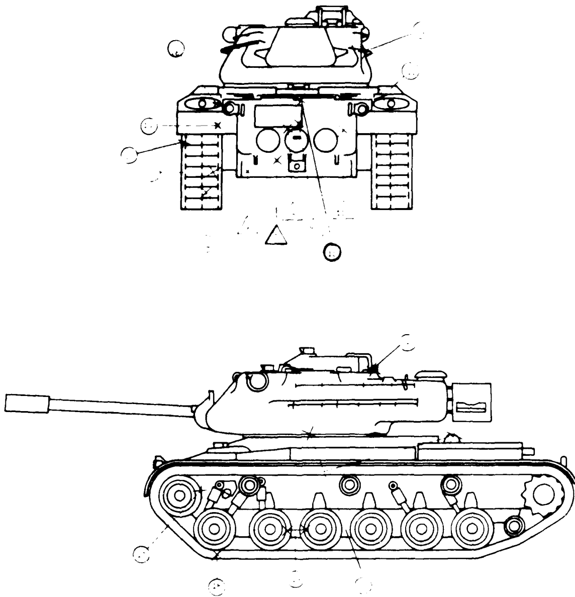
FIGURE 7. Impact Diagram, Target 2.
