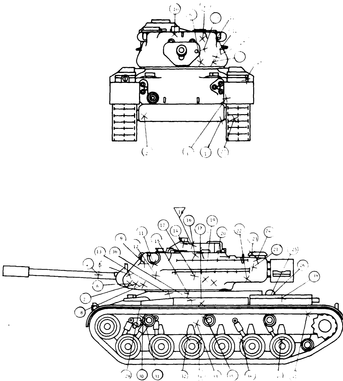
FIGURE 106. Impact Diagram, Target 41.
