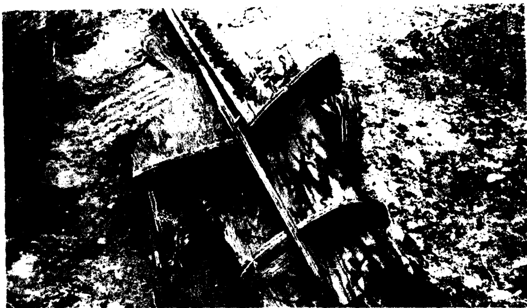
FIGURE 75. Loader Manikin, Target 35, Showing Damage from Perforations into the Fighting Compartment.
