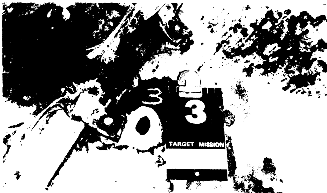
Figure 12. Impact Three, Target 11. The photograph shows the bolt on roadwheel 11.
