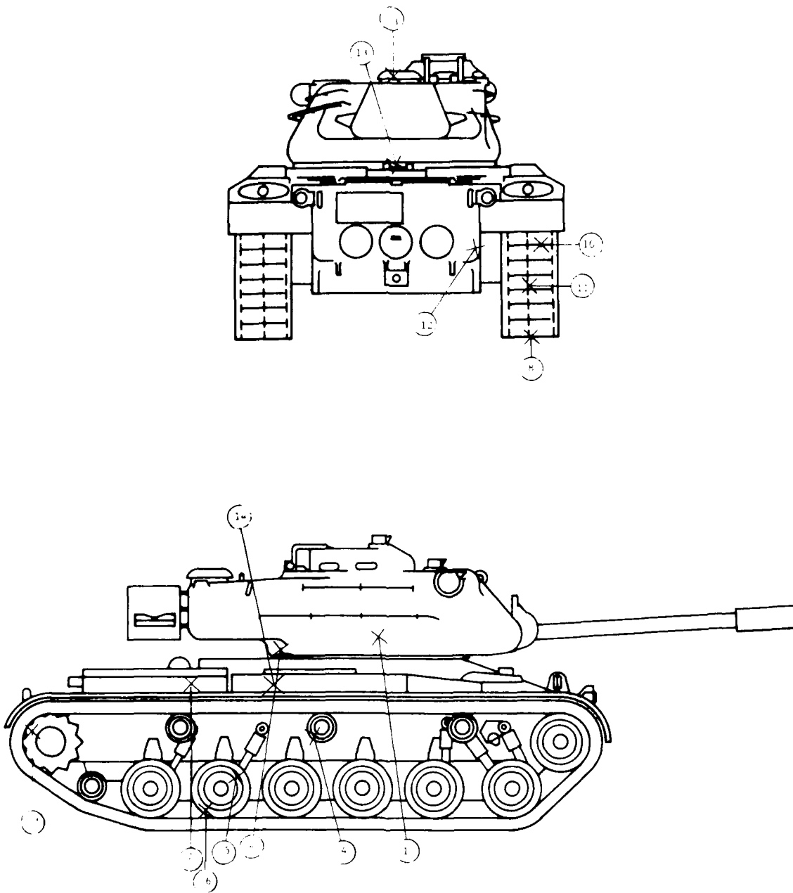
FIGURE 15. Impact Diagram, Target 7.
