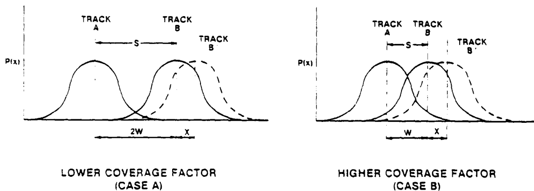
Figure 4-2. Effect of Deviations from Track on POD
