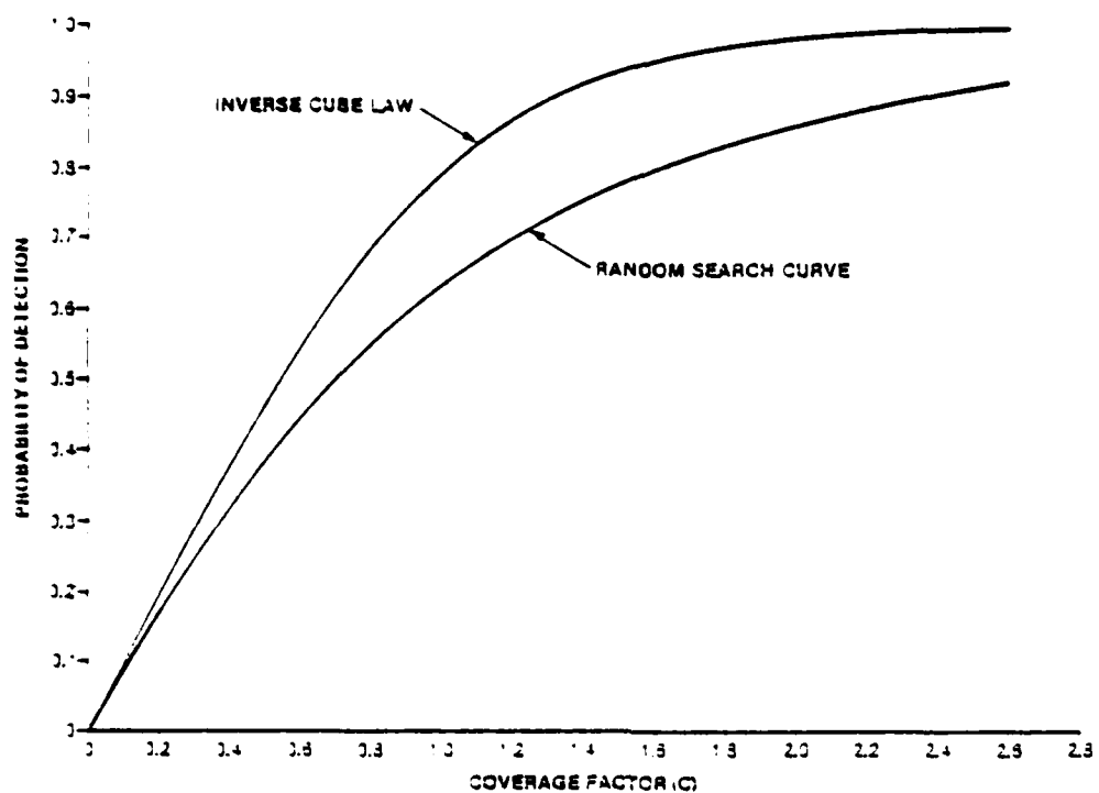
Figure 1-5. Comparison of Inverse Cube Law and Uniform Random Search Models
