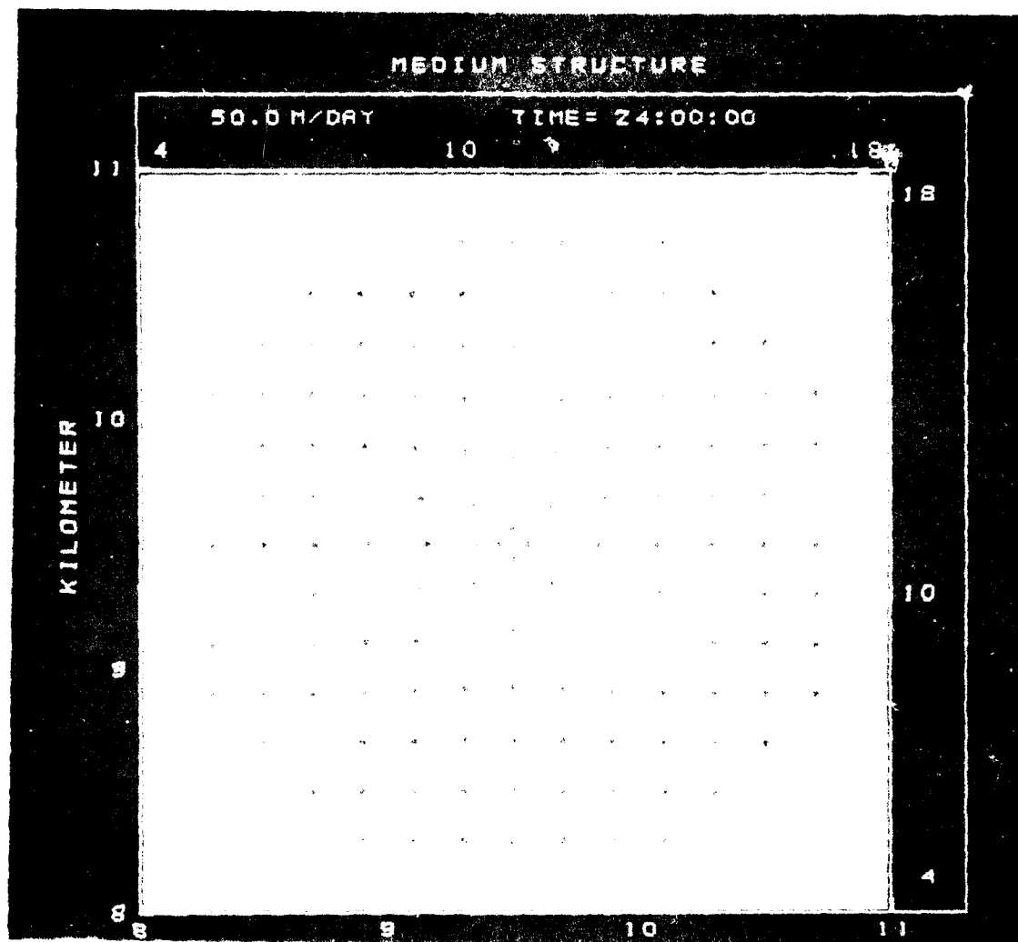
Figure B-8. Computed constant drawdown contours (0.2 m drawdown steps) and average-velocity field after 24 hours pumping medium-structured virgin aquifer at a constant rate of 120 m 3 /h.
