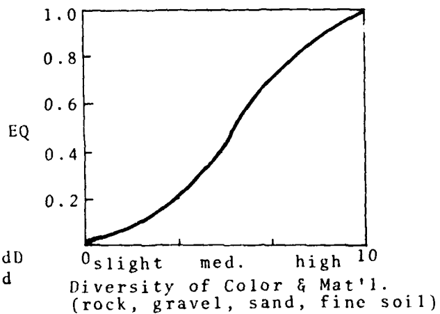
FIGURE 45. GEOLOGIC SURFACE MATERIAL
