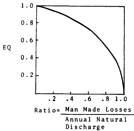
FIGURE 19. BASIN HYDROLOGIC LOSS
