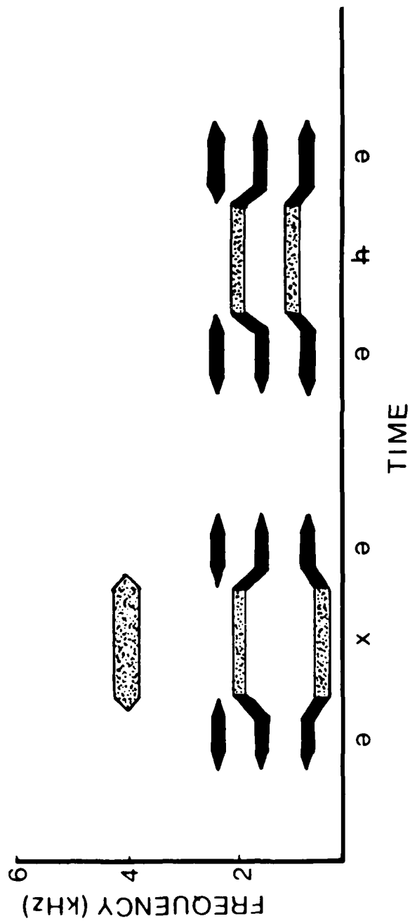
Figure 2. Schematic spectrograms of stimulus #1 (on left) and of stimulus #12 (on right) in the synthetic /x/-/h/ series.
