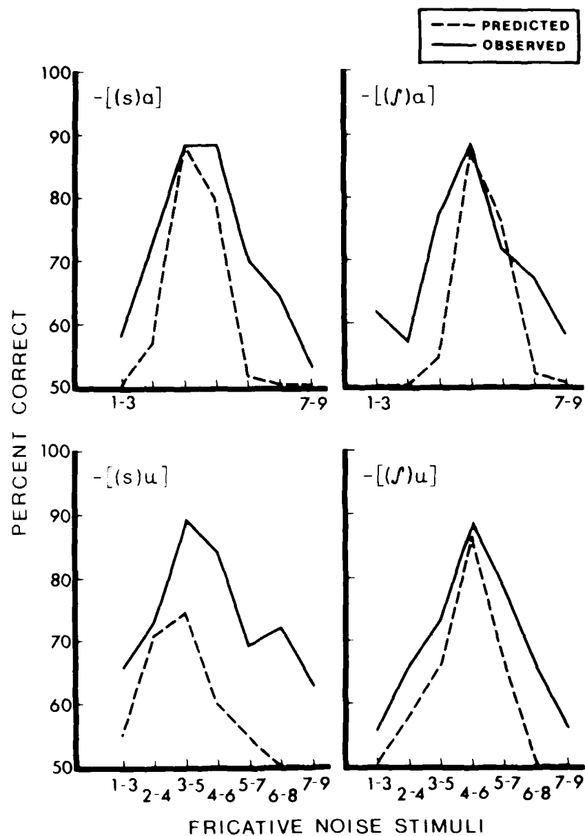
Figure 2. AXB discrimination performance of six "categorical" subjects: Two-step comparisons of [f]-[s] noises in four different vocalic contexts.
