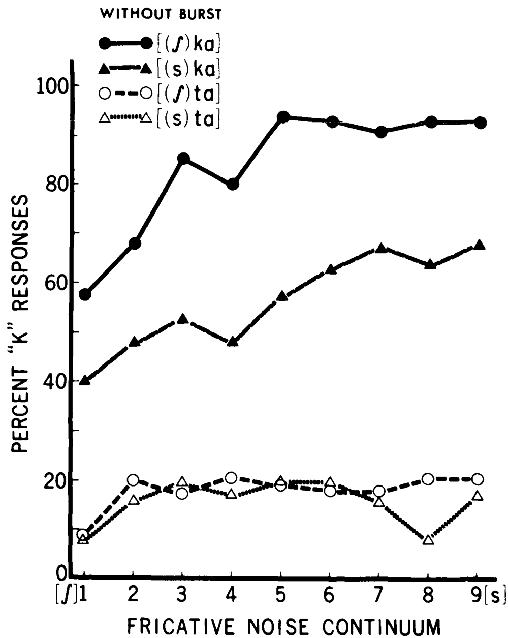
Figure 4. Effects of (synthetic) fricative noise spectrum on stop identification in CV portions excerpted from different fricative contexts (Exp. 2C).
