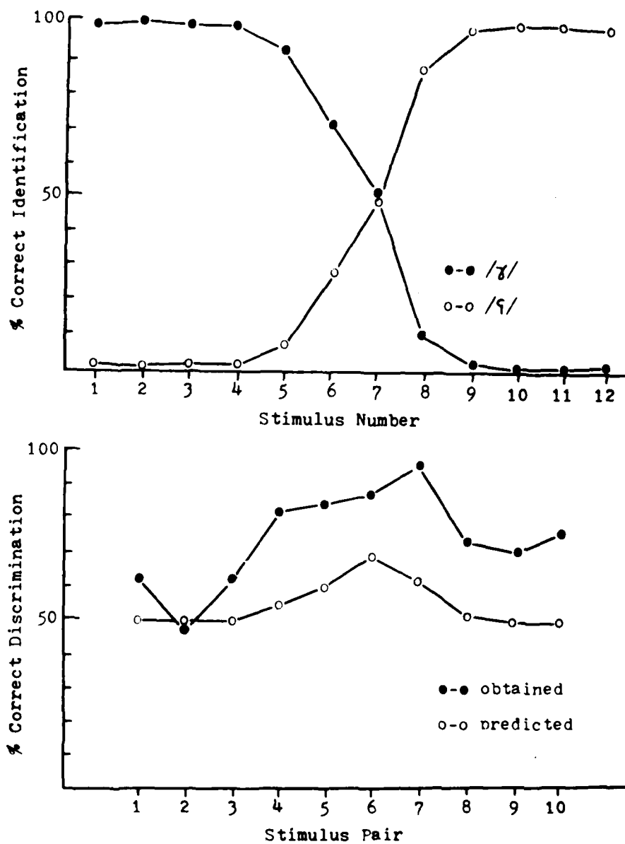
Figure 6. Identification function (top) and predicted and obtained discrimination functions (bottom) for seven subjects for the /ɣ/-/ɣ/ series.
