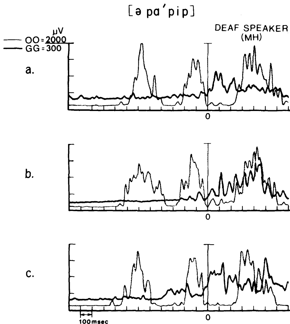
Figure 11. A single selected token of the EMG potential from the genioglossus and orbicularis oris muscles as produced by the deaf speaker. The vertical line indicates the acoustic release of the /p/ closure. In Figure 11a, peak genioglossus activity occurs between the second and third orbicularis oris peaks, but is late relative to the acoustic event. This pattern was most like normal. In Figure 11b and 11c, the single tokens show that genioglossus activity was either too late or too early respectively. (N.B. Single tokens filtered with settings used for the average in Figure 8.)
