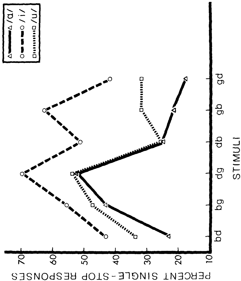
Figure 4. Percent single-stop responses (averaged over all silence durations) to the 18 VC 1 -C 2 V combinations (natural speech).
