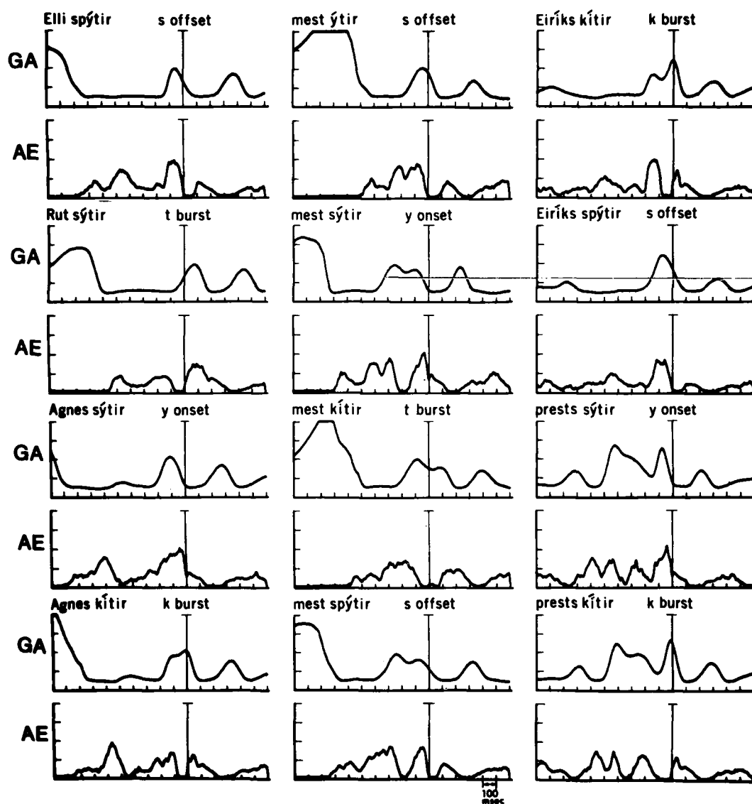
Figure 3. Glottal area and audio signals for 12 utterances containing different obstruent clusters.
