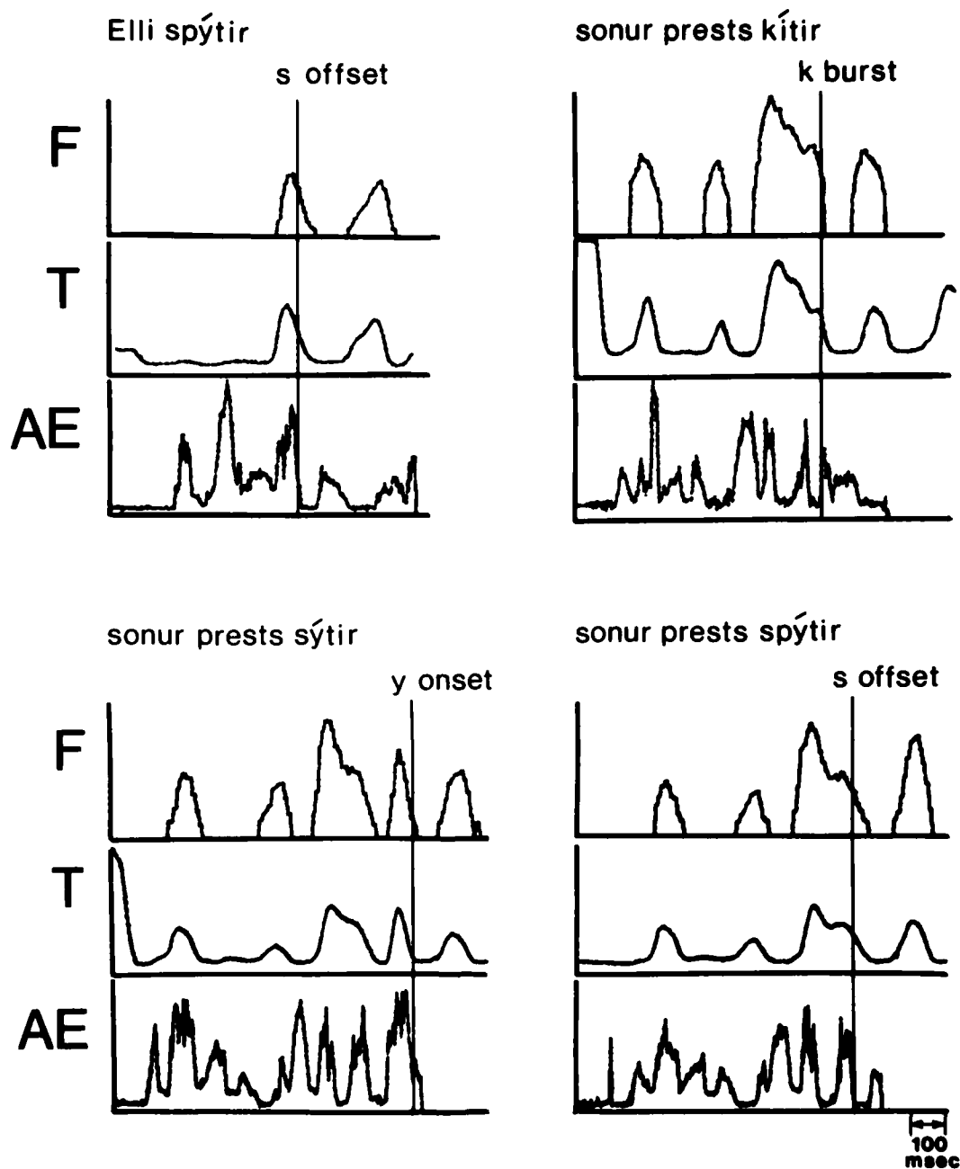
Figure 1. Comparisons of fiberoptic and transillumination records for four utterances. F = glottal area obtained by fiberoptic filming. T = glottal area obtained by transillumination. AE = audio envelope.
