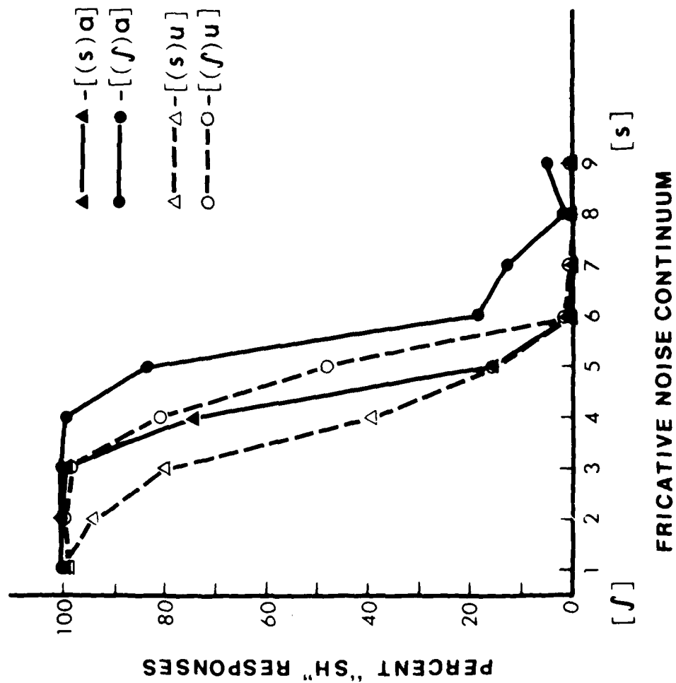
Figure 1. Identification functions for a [ʃ]-[s] noise continuum in four different vocalic contexts.
