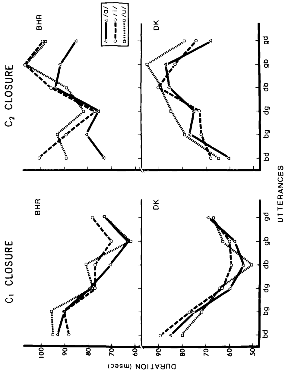
Figure 3. Average C 1 and C 2 closure durations in 18 VC 1 -C 2 V combinations produced by two speakers.
