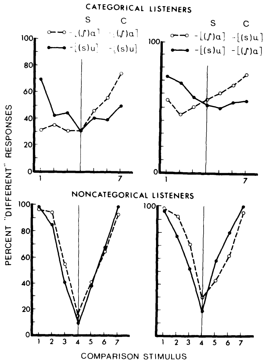
Figure 3. Fixed-standard AX discrimination performance of eight "categorical" subjects (upper panels) and five "noncategorical" subjects (lower panels): Percent "different" responses to pairings of a standard (S, stimulus No. 4) with seven comparison (C) stimuli, in four different vocalic context conditions.
