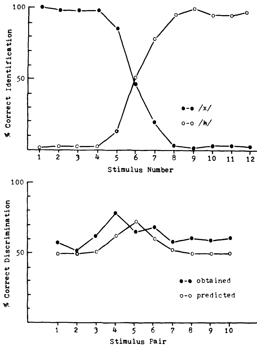
Figure 5. Identification function (top) and predicted and obtained discrimination functions (bottom) for seven subjects for the /x/-/h/ series.
