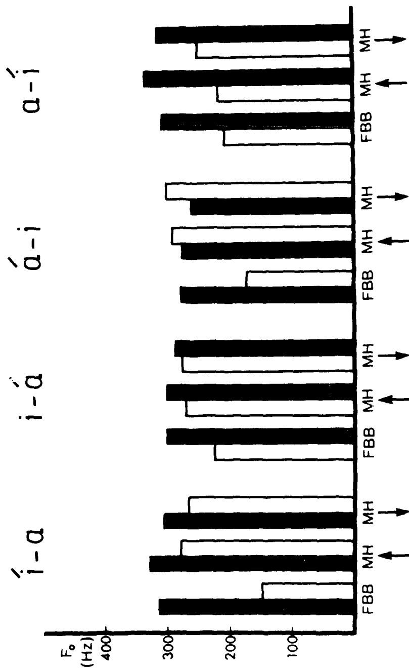
Figure 3. Mean fundamental frequency ( F_0 ) for the hearing and deaf speaker.
