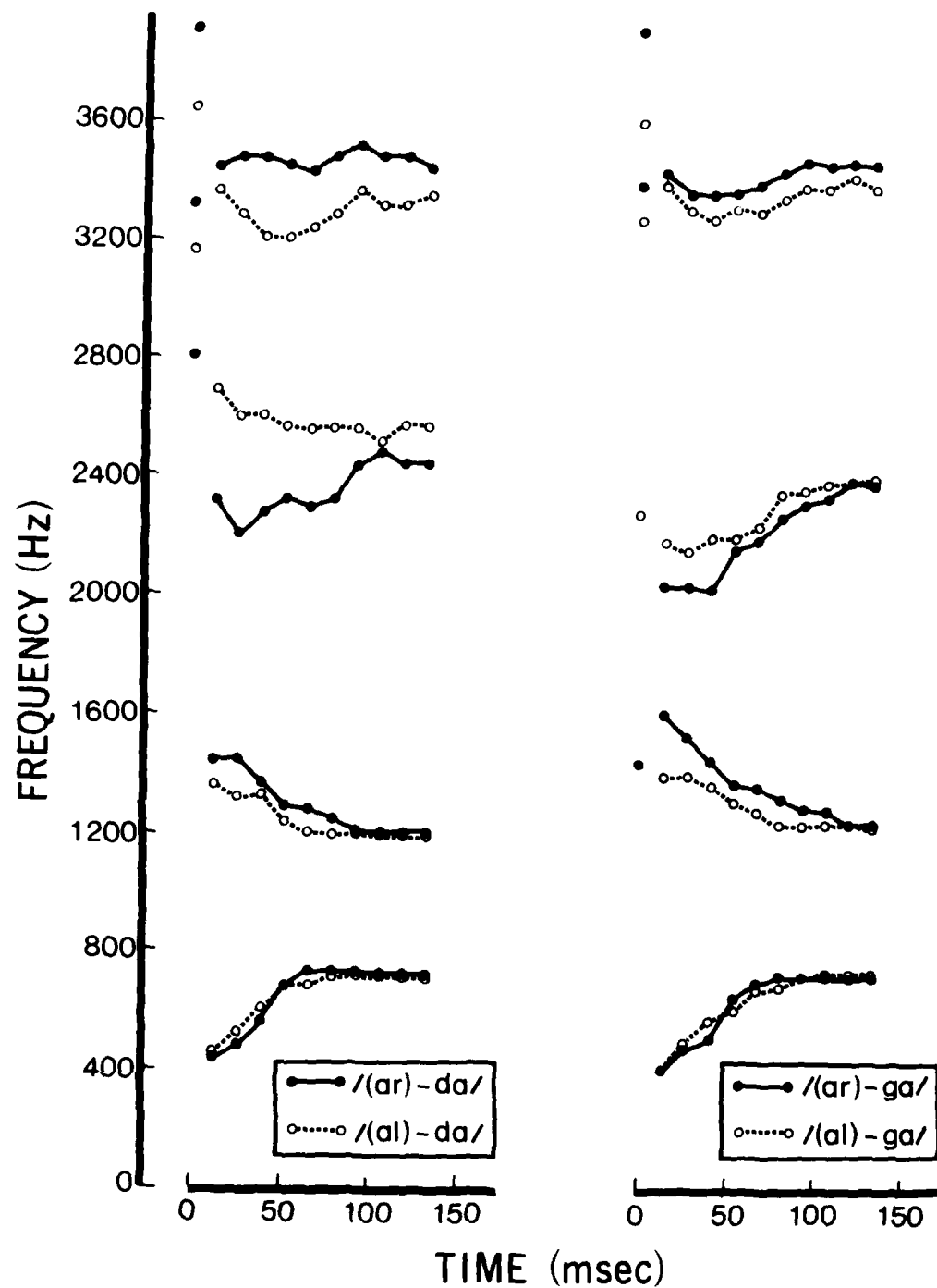
Figure 4. Average formant values for the first 145 msec of natural [da] and [ga], plotted separately for tokens produced after [al] and [ar].
