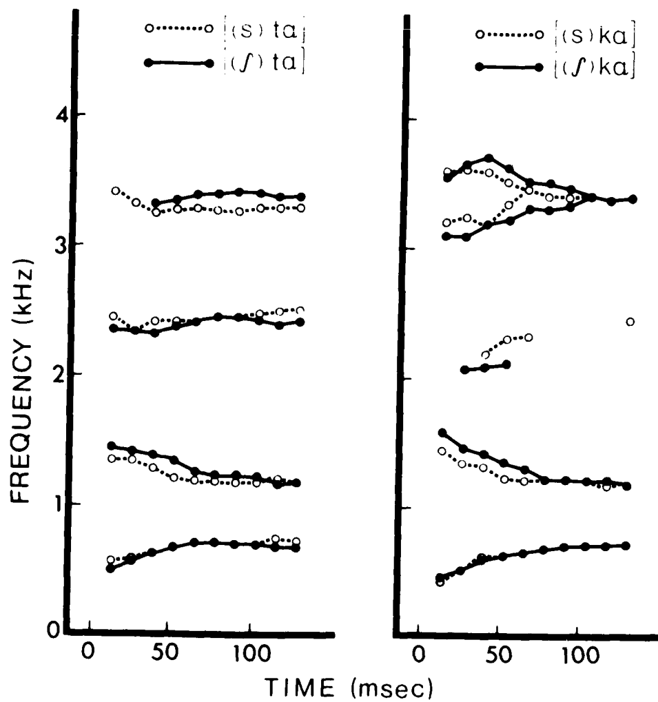
Figure 7. Average spectral structure of CV portions in different fricative contexts (Exp. 2).
