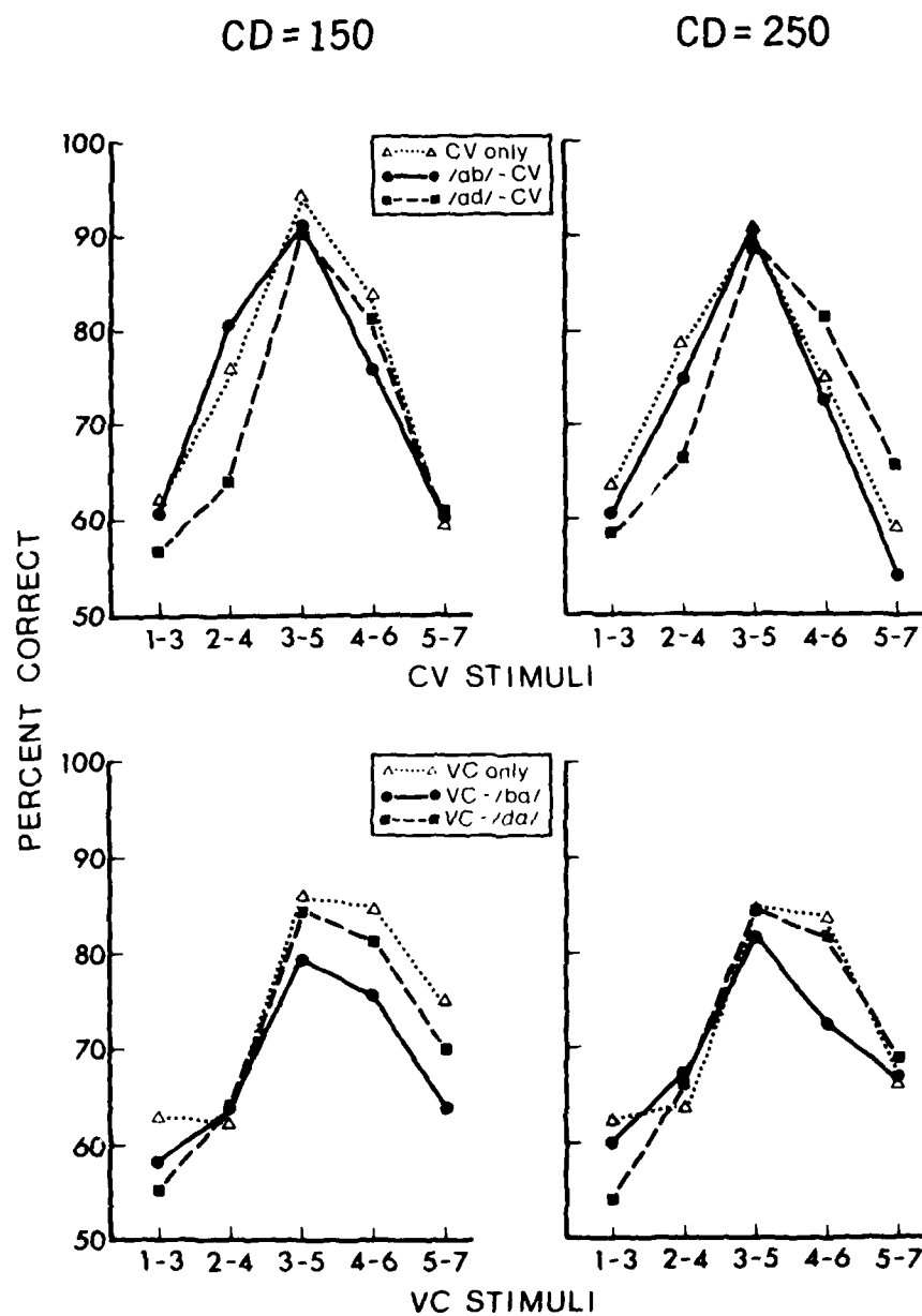
Figure 3. AXB discrimination performance for VC and CV stimuli in isolation and in context, as a function of context stimulus and closure duration (Exp. 2).
