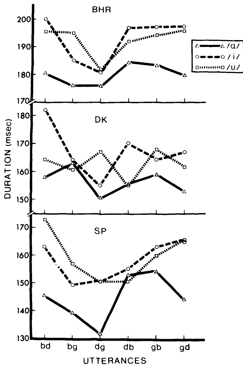
Figure 2. Average total closure durations in 18 VC 1 -C 2 V combinations produced by three speakers.
