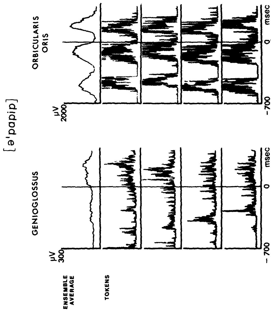
Figure 8. /ə'pəpɪp/ as produced by a deaf speaker. Data presented as in Figure 6.
