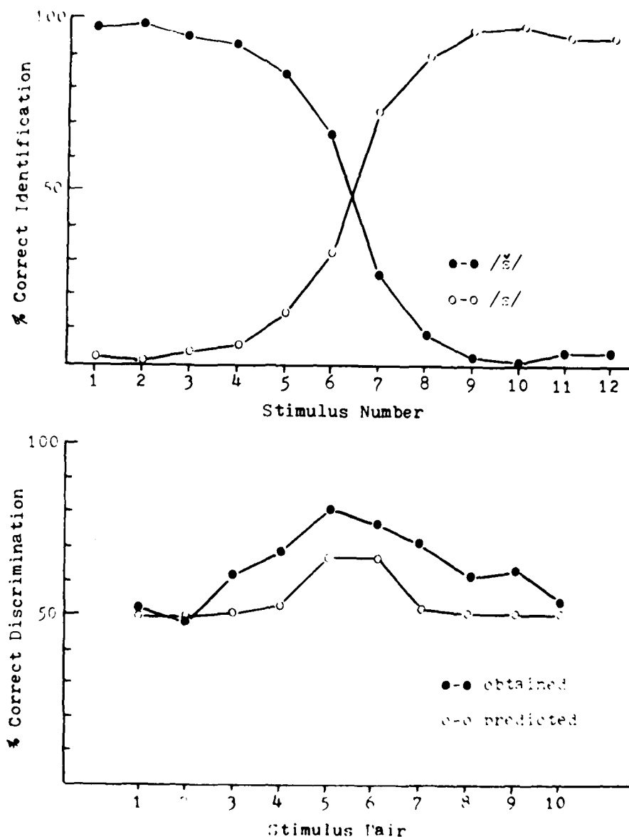
Figure 4. Identification function (top) and predicted and obtained discrimination functions (bottom) for seven subjects for the /s/-/ʃ/ series.
