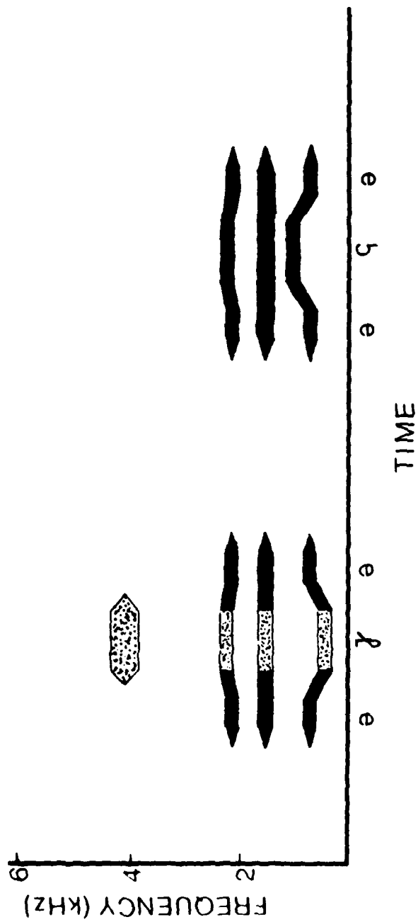
Figure 3. Schematic spectrograms of stimulus #1 (on left) and of stimulus #12 (on right) in the synthetic /γ/-/γ/ series.
