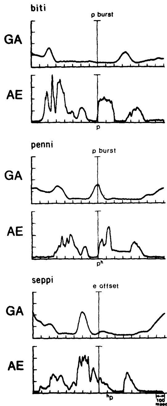
Figure 2. Average transillumination signal (GA), and audio envelope (AE) for utterances containing unaspirated (top), postaspirated (middle), and preaspirated (bottom) stops.
