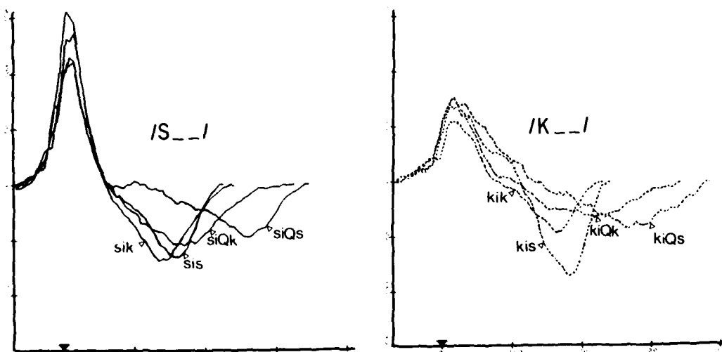
Figure 7. Superimposed curves of the first derivative of the averaged glottograms for all the test voiceless sequences.
