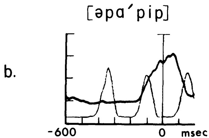
Figure 10. Ensemble average of the EMG potentials for genioglossus and orbicularis oris for the utterance type /əpapip/ produced by the hearing speaker. The vertical line indicates the acoustic release of the /p/ closure.
