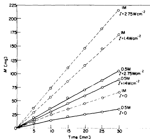
Fig. 1 Variation of the amount of material diffused as a function of time
