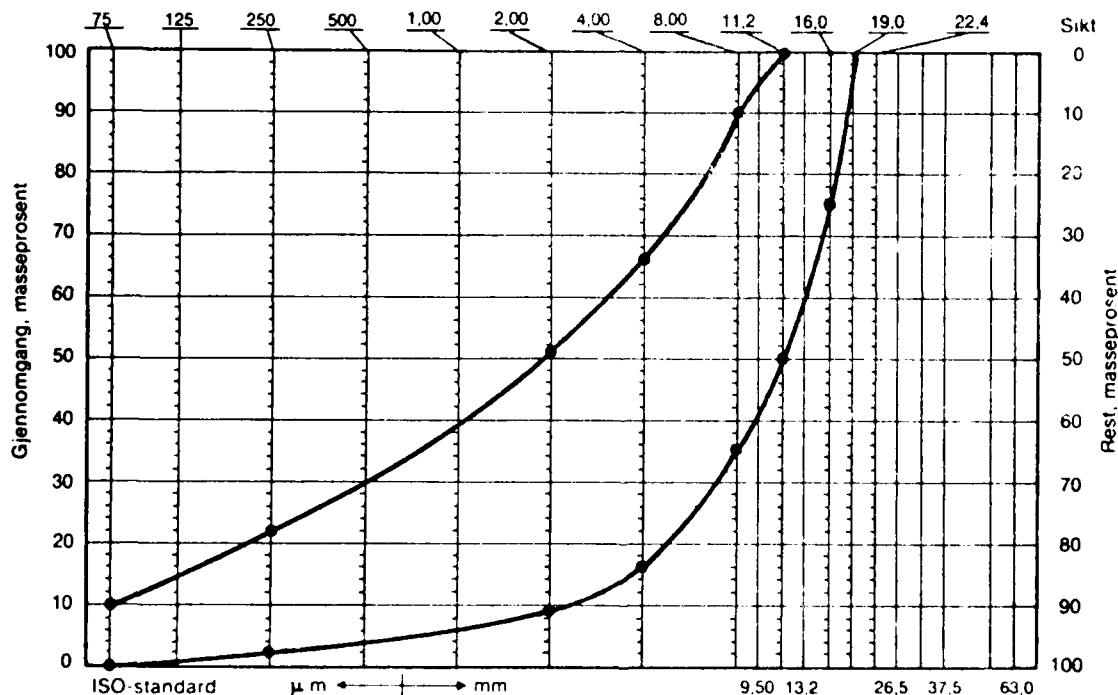
FIGURE 10: Grading limits for surface dressing with gravel, so-called "Ottadekke" [Otta-cover]. [Top right of figure: Sieve. Vertically at left: Passing through, percentage of mass. Vertically at right: Remaining, percentage of mass.]
