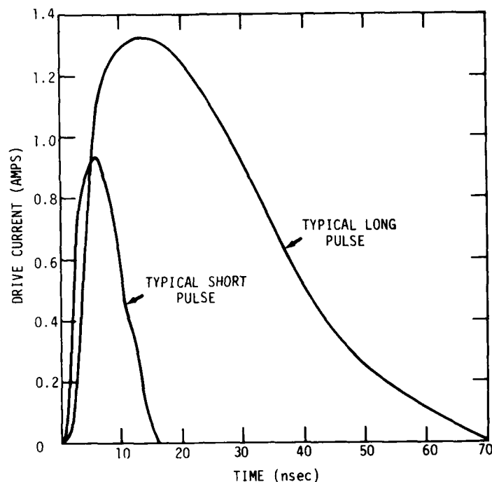
Figure 26. Typical short and long pulse current waveforms
