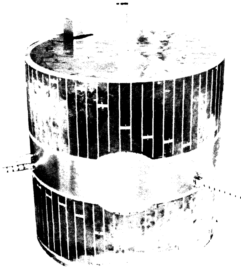
Figure 14. SCATSAT side view
