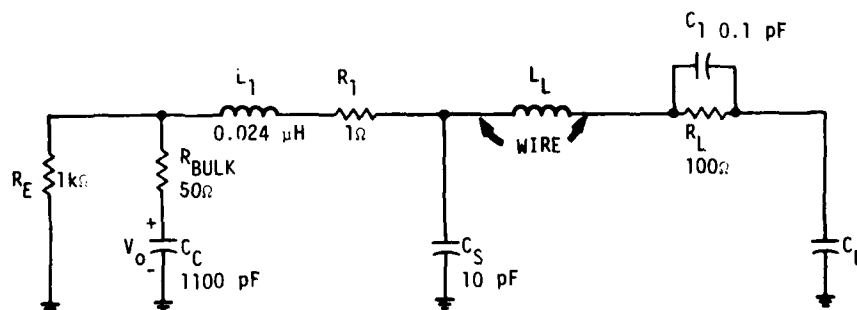
Figure B-1. Equivalent electrical circuit as modeled for TRAC
