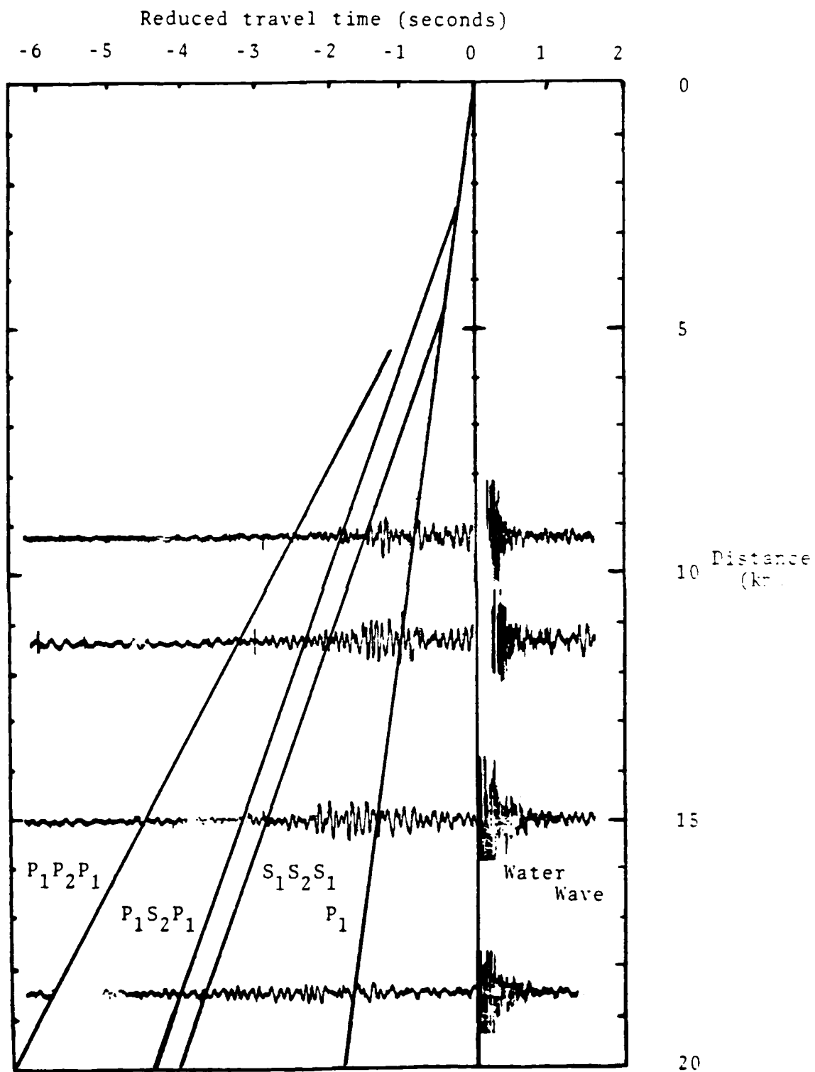
Figure 3 Reduced Travel Time-Distance Plot, Geophone 3X (Mid-depth Shots)
