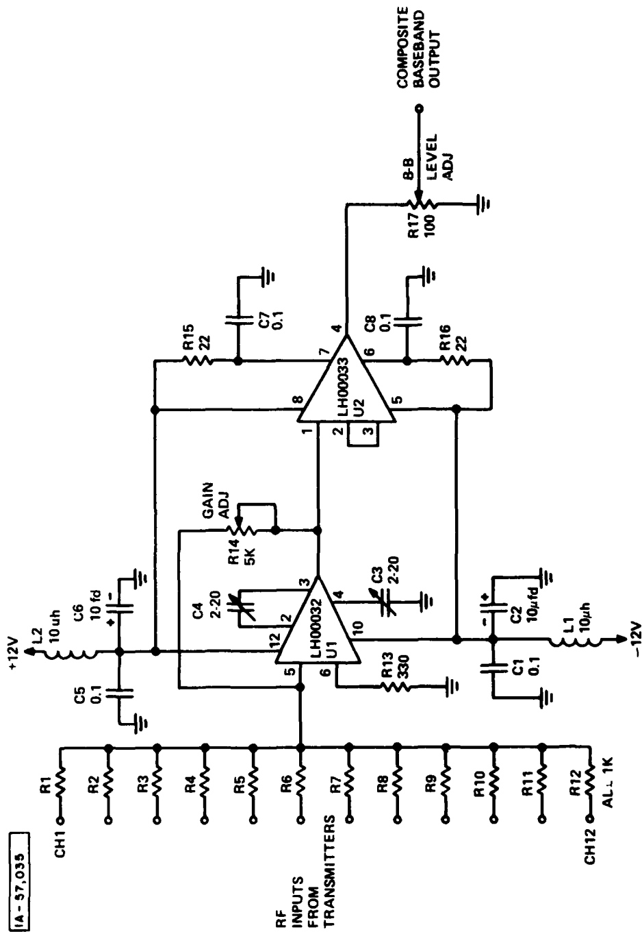
Figure 5. Schematic of Summing Amplifier Circuits
