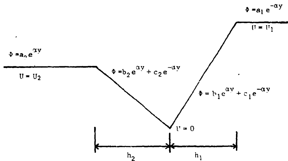
Fig. 29.- Straight line approximation for the wake profile of the splitter plate. Expressions are the perturbation amplitudes for the stream function.
