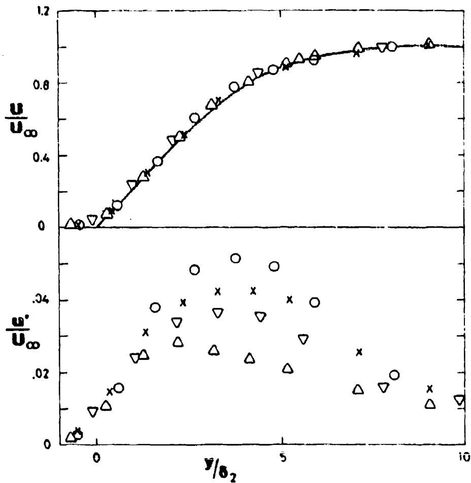
Fig. 17.- Nondimensional profiles of boundary layer at several spanwise locations. O , z = -35 mm; X , z = -25 ; ▽ , z = 15 ; Δ , z = -5 . Solid line is Blasius profile. Layer II, x = 1 mm.
