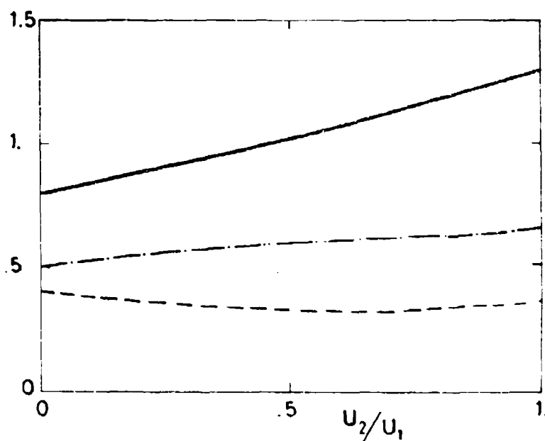
Fig. 31.- Properties of most spatially amplified wave above. — \alpha h_1 ; --- c_r/u_1 ; - - - \alpha h_1 c_1/c_r .
