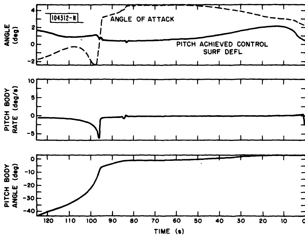
Fig. 4.4(c). Sample output for glide bomb.
