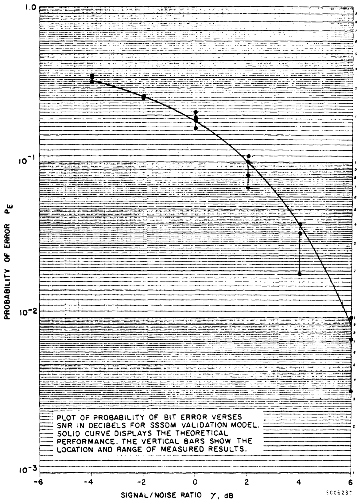
Figure 4-1. SSSDM Probability of Bit Error Vs SNR
