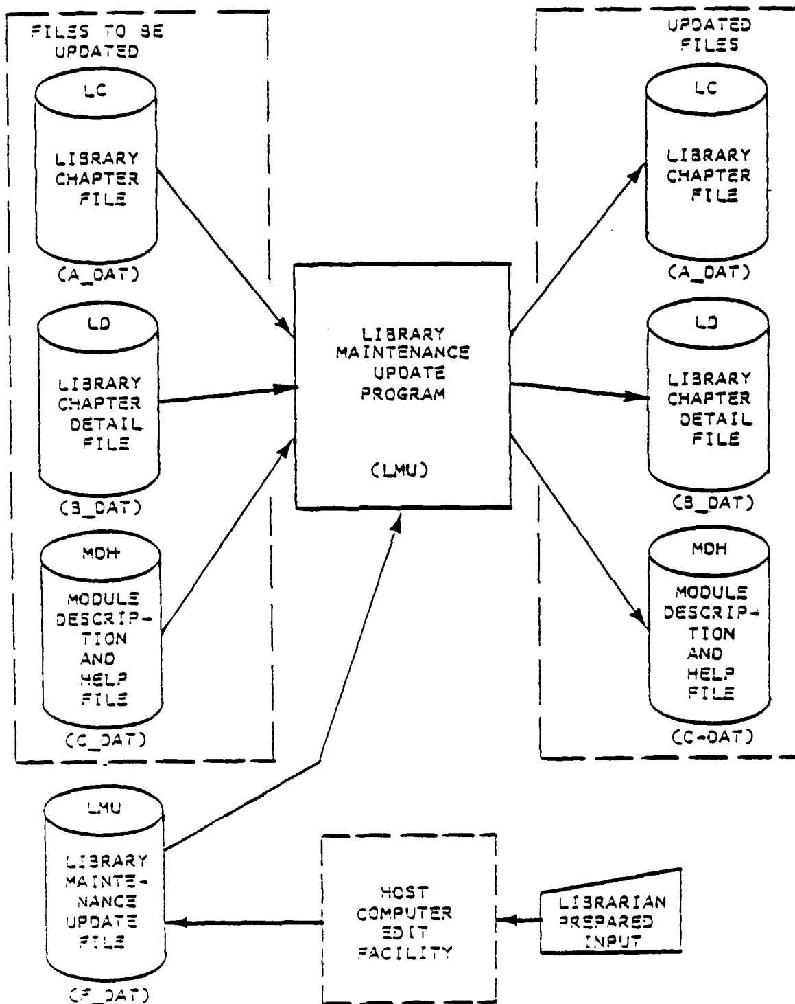
Figure 3-35. Structure of Maintenance/Update (MU) Subsystem
