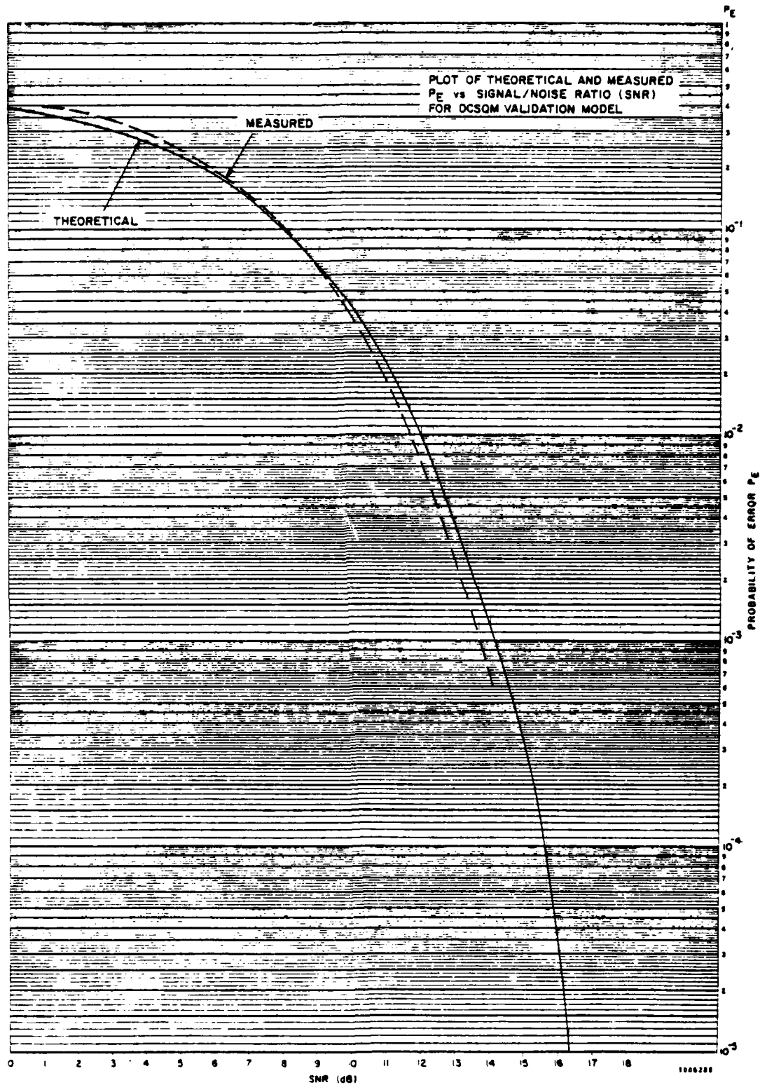
Figure 4-2. DCSQM Probability of Bit Error Vs SNR
