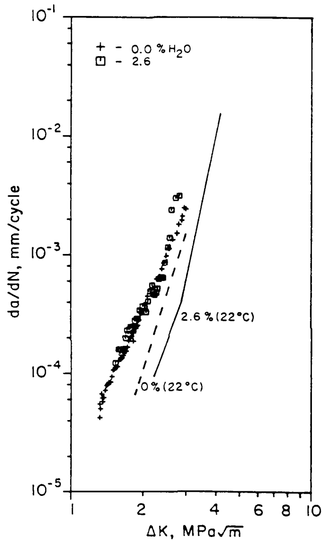
Figure 12 - Crack growth rates in N66 tested at 52^\circ\text{C} . Lines represent FCP behavior at 22^\circ\text{C} . Note greater shift in the 2.6% \text{H}_2\text{O} material as compared to dry N66.
