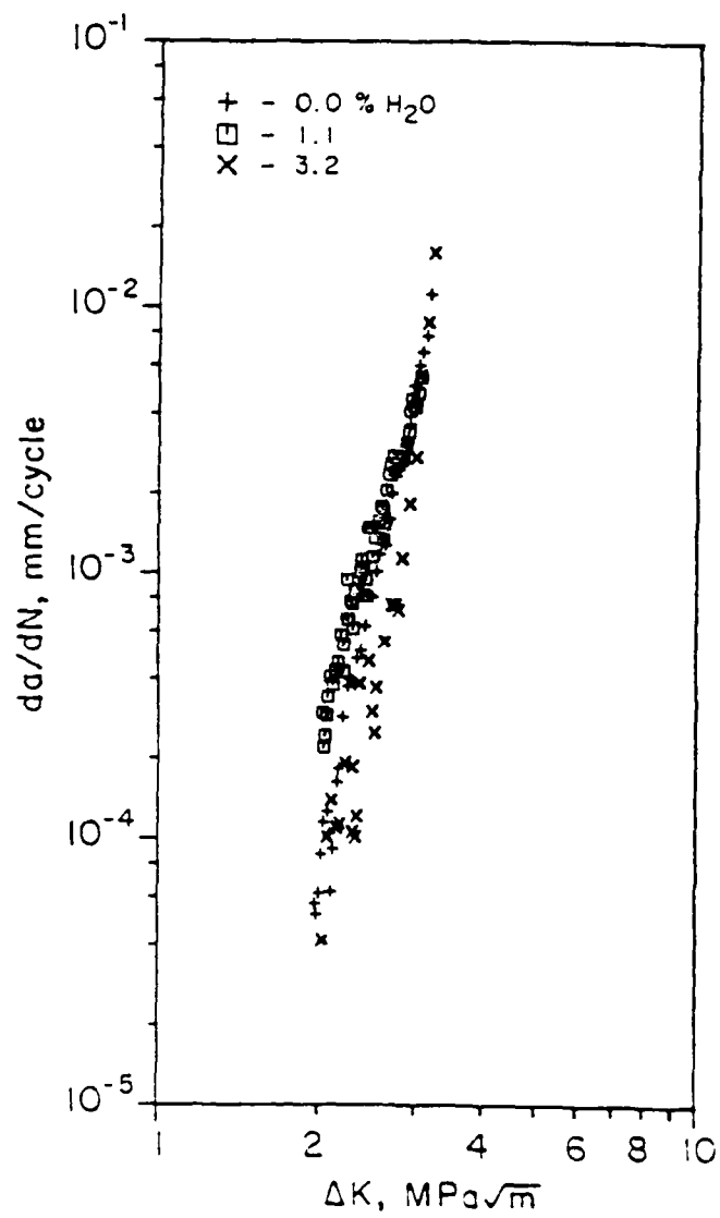
Figure 5 - Effect of moisture on fatigue crack growth rates in N612.
