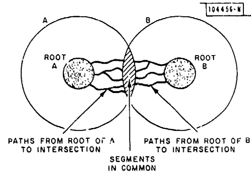
Fig. IV-4. The intersection of two equivalence classes.
